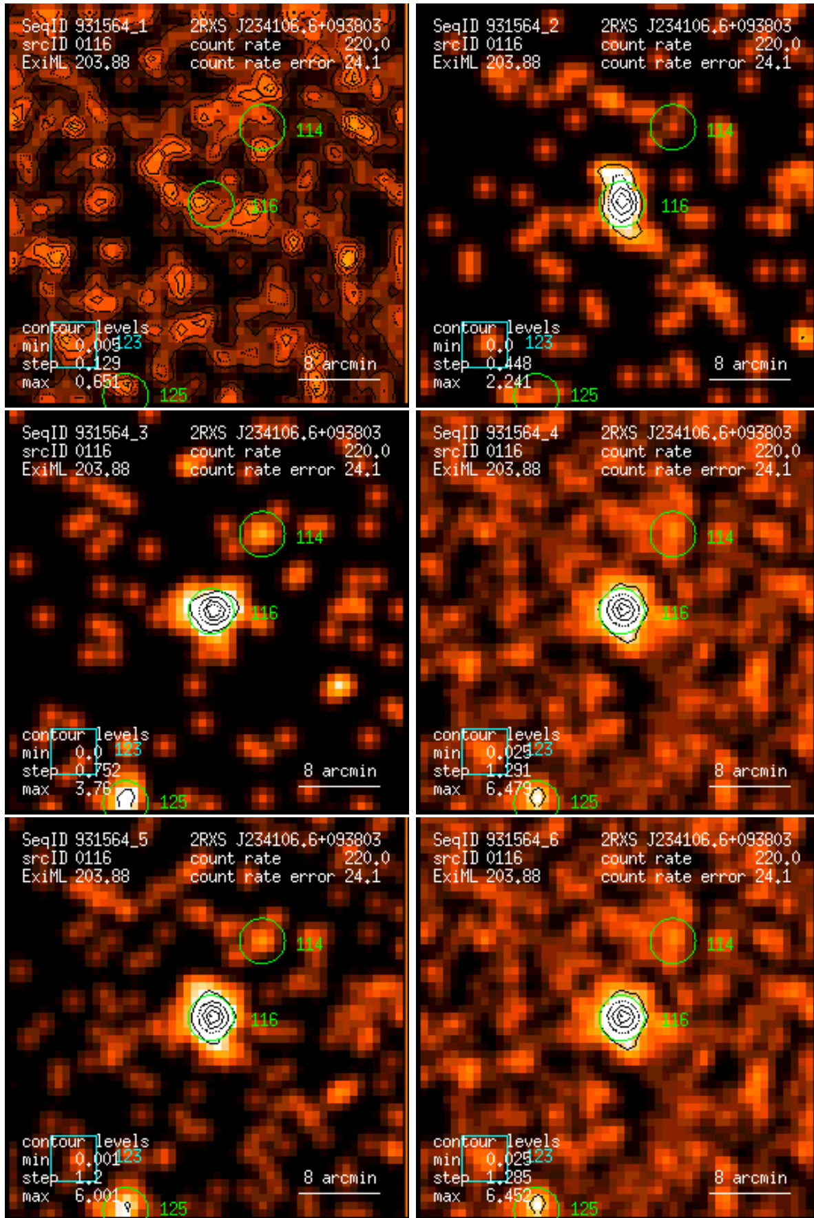
Figure 116: RASS 931564: detection 0116: band rate images, Gaussian filter: (1) PSPC channels 11 – 41, (2) 52 – 90, (3) 91 – 201, (4) 11 – 235, (5) 52 – 201, (6) 11 – 201. Broad band rates in counts/ks. Band rate contour levels in counts/ks/arcmin 2 .
