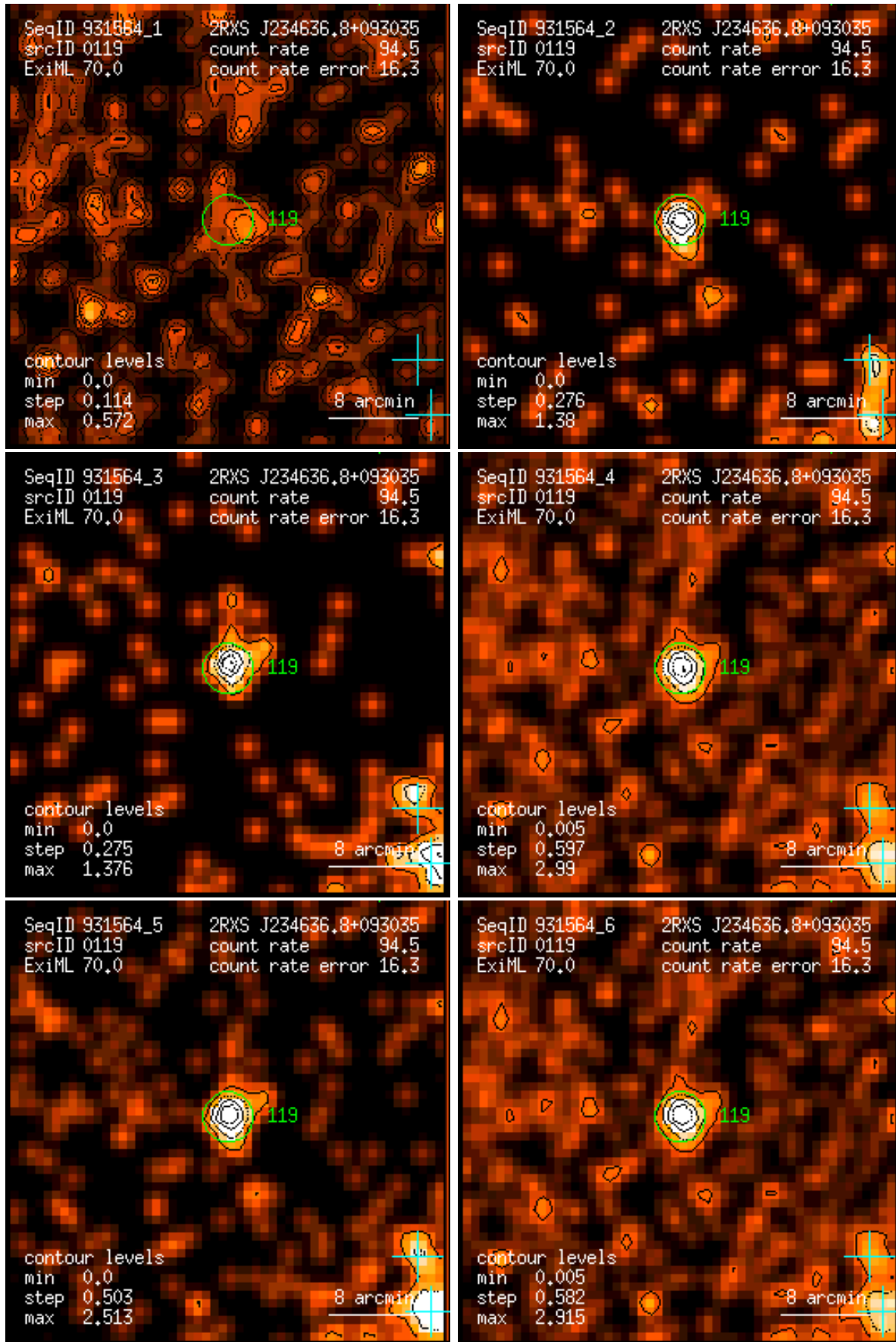
Figure 119: RASS 931564: detection 0119: band rate images, Gaussian filter: (1) PSPC channels 11 – 41, (2) 52 – 90, (3) 91 – 201, (4) 11 – 235, (5) 52 – 201, (6) 11 – 201. Broad band rates in counts/ks. Band rate contour levels in counts/ks/arcmin 2 .
