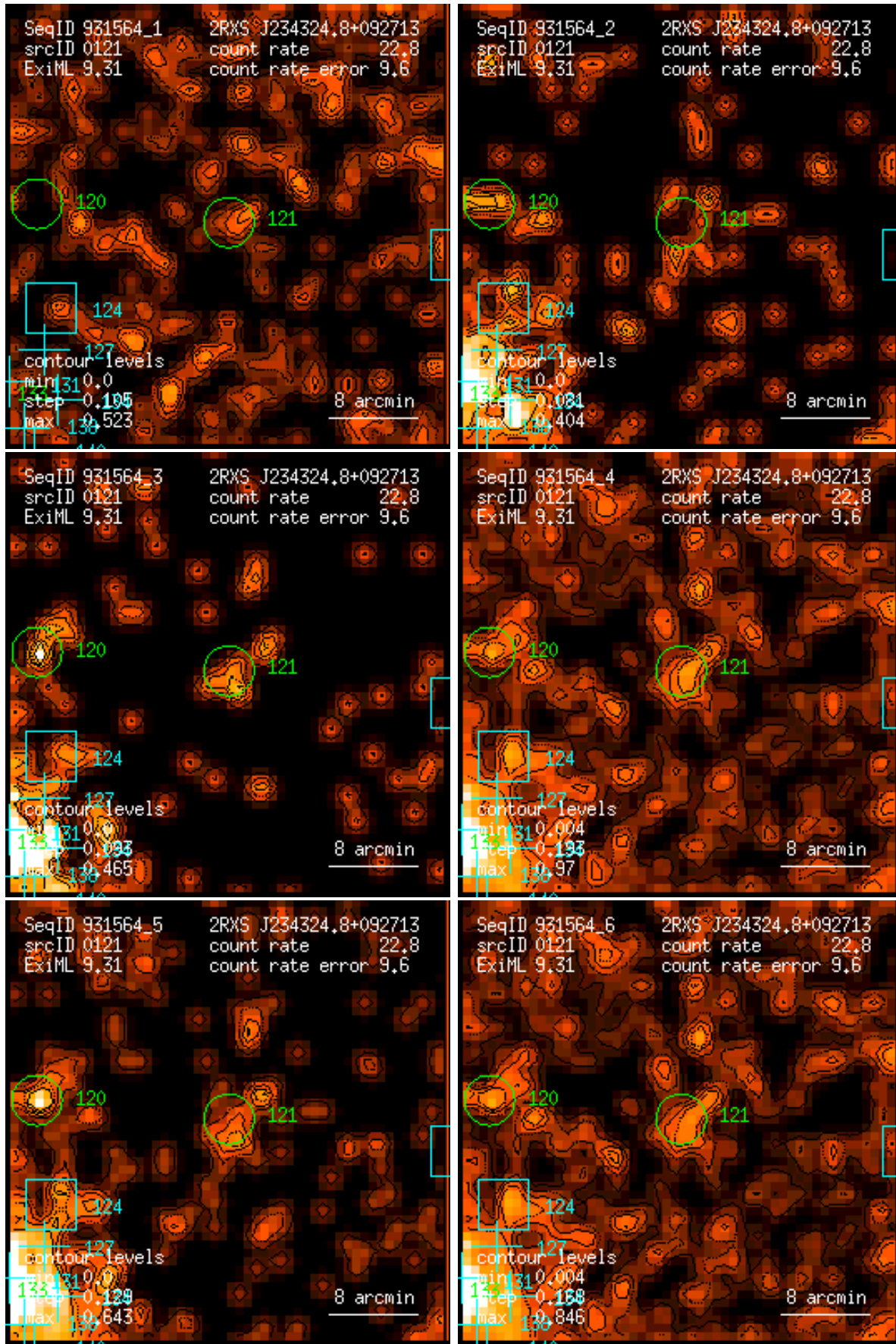
Figure 121: RASS 931564: detection 0121: band rate images, Gaussian filter: (1) PSPC channels 11 – 41, (2) 52 – 90, (3) 91 – 201, (4) 11 – 235, (5) 52 – 201, (6) 11 – 201. Broad band rates in counts/ks. Band rate contour levels in counts/ks/arcmin 2 .
