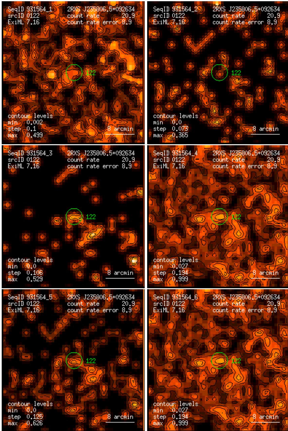
Figure 122: RASS 931564: detection 0122: band rate images, Gaussian filter: (1) PSPC channels 11 – 41, (2) 52 – 90, (3) 91 – 201, (4) 11 – 235, (5) 52 – 201, (6) 11 – 201. Broad band rates in counts/ks. Band rate contour levels in counts/ks/arcmin 2 .
