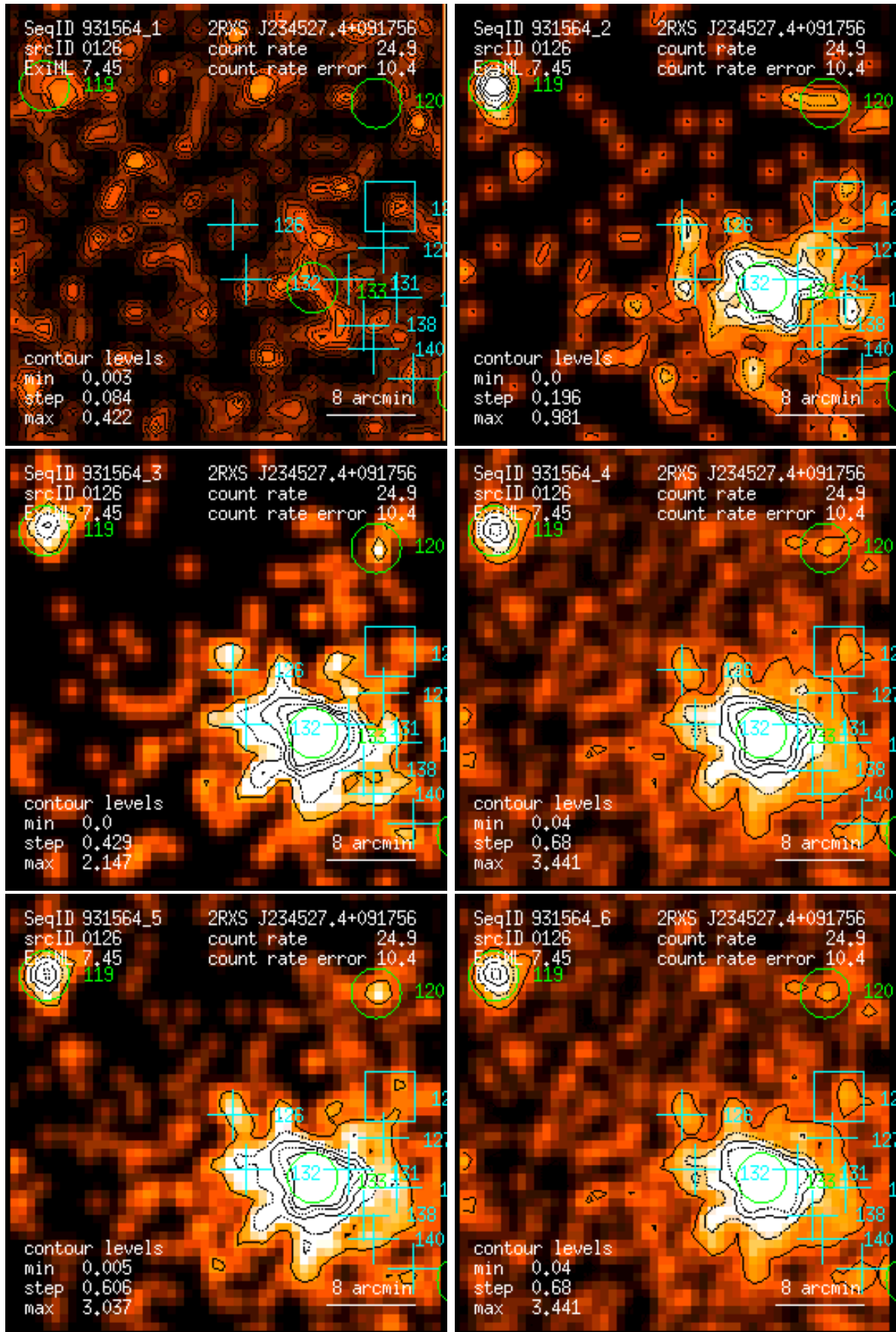
Figure 126: RASS 931564: detection 0126: band rate images, Gaussian filter: (1) PSPC channels 11 – 41, (2) 52 – 90, (3) 91 – 201, (4) 11 – 235, (5) 52 – 201, (6) 11 – 201. Broad band rates in counts/ks. Band rate contour levels in counts/ks/arcmin 2 .
