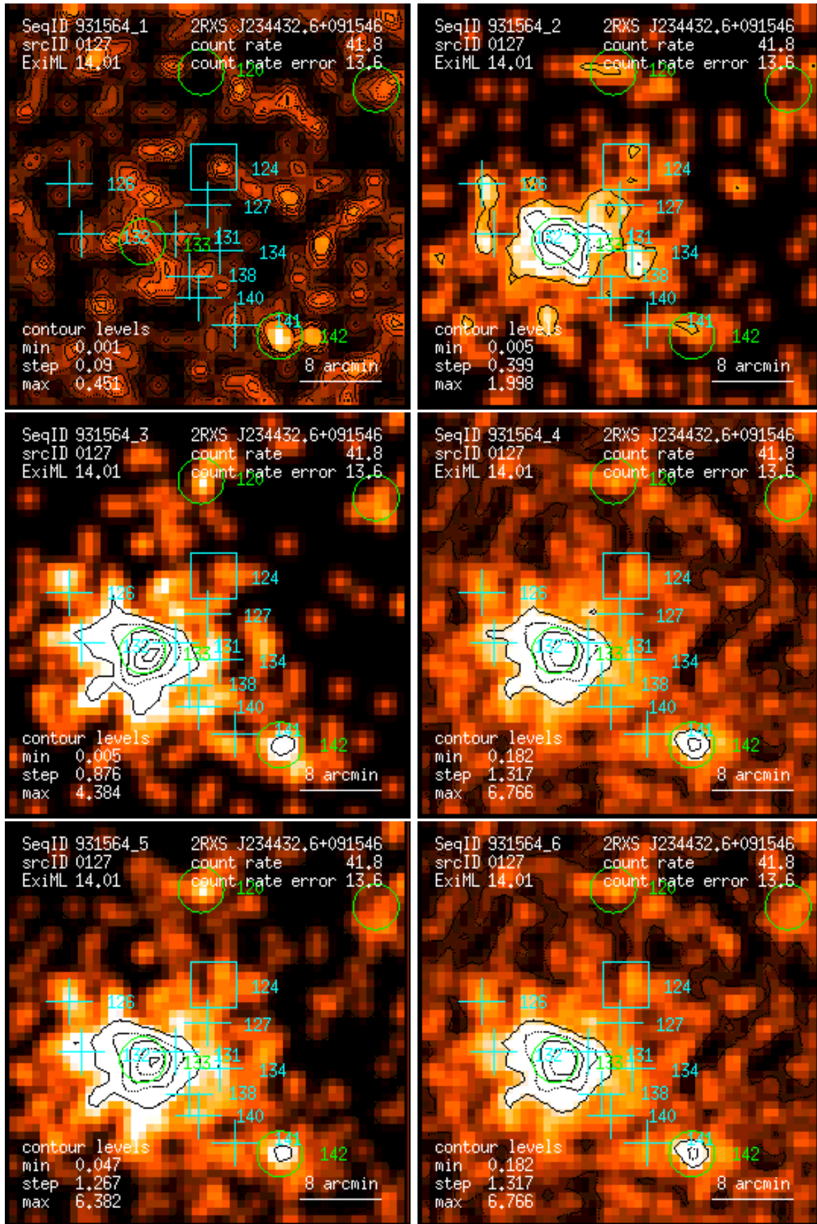
Figure 127: RASS 931564: detection 0127: band rate images, Gaussian filter: (1) PSPC channels 11 – 41, (2) 52 – 90, (3) 91 – 201, (4) 11 – 235, (5) 52 – 201, (6) 11 – 201. Broad band rates in counts/ks. Band rate contour levels in counts/ks/arcmin 2 .
