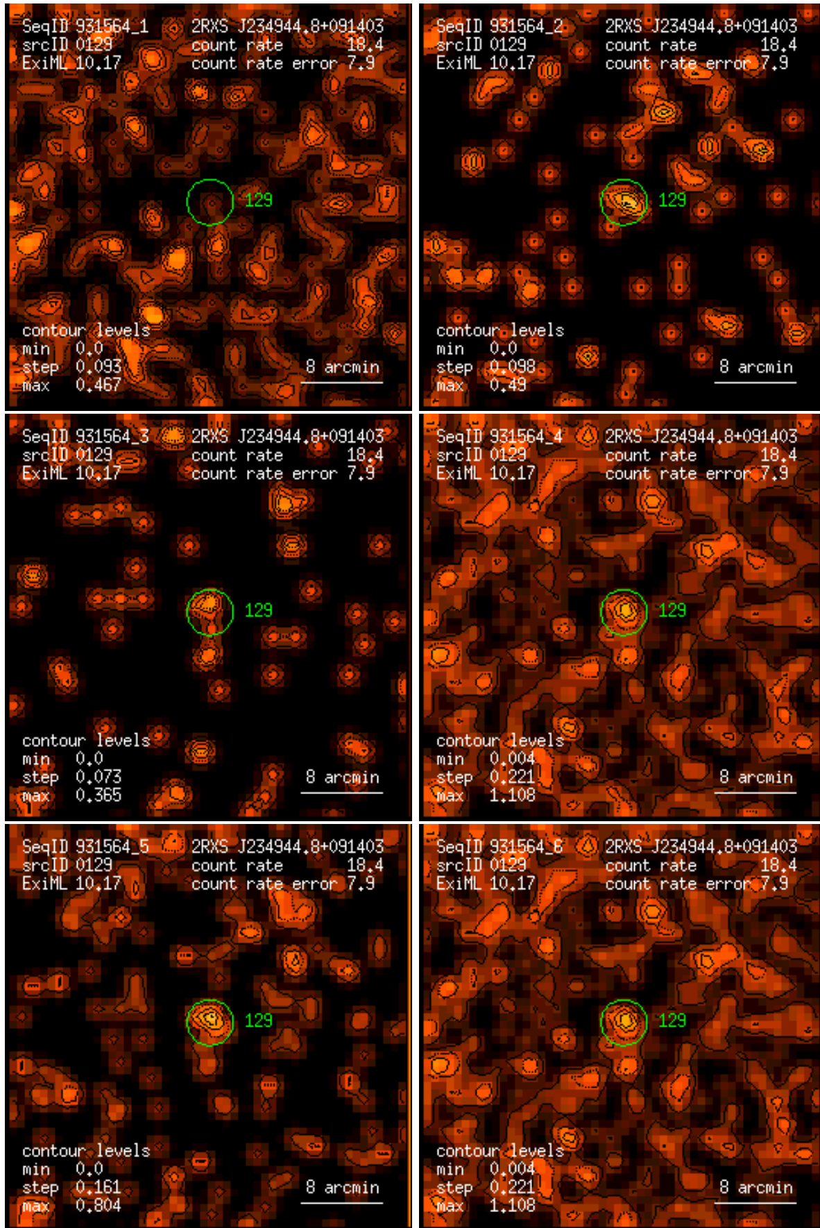
Figure 129: RASS 931564: detection 0129: band rate images, Gaussian filter: (1) PSPC channels 11 – 41, (2) 52 – 90, (3) 91 – 201, (4) 11 – 235, (5) 52 – 201, (6) 11 – 201. Broad band rates in counts/ks. Band rate contour levels in counts/ks/arcmin 2 .
