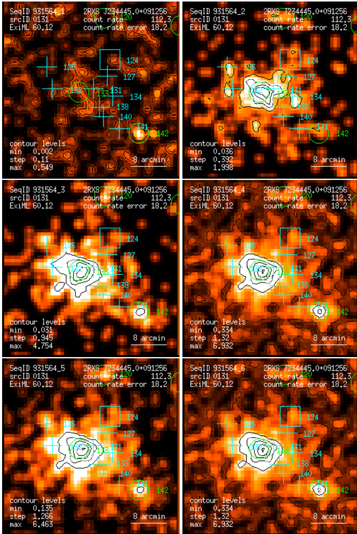
Figure 131: RASS 931564: detection 0131: band rate images, Gaussian filter: (1) PSPC channels 11 – 41, (2) 52 – 90, (3) 91 – 201, (4) 11 – 235, (5) 52 – 201, (6) 11 – 201. Broad band rates in counts/ks. Band rate contour levels in counts/ks/arcmin 2 .
