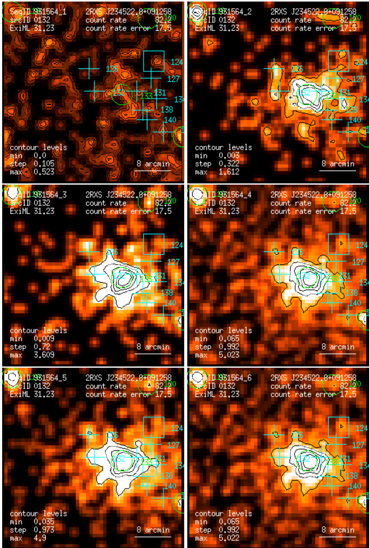
Figure 132: RASS 931564: detection 0132: band rate images, Gaussian filter: (1) PSPC channels 11 – 41, (2) 52 – 90, (3) 91 – 201, (4) 11 – 235, (5) 52 – 201, (6) 11 – 201. Broad band rates in counts/ks. Band rate contour levels in counts/ks/arcmin 2 .
