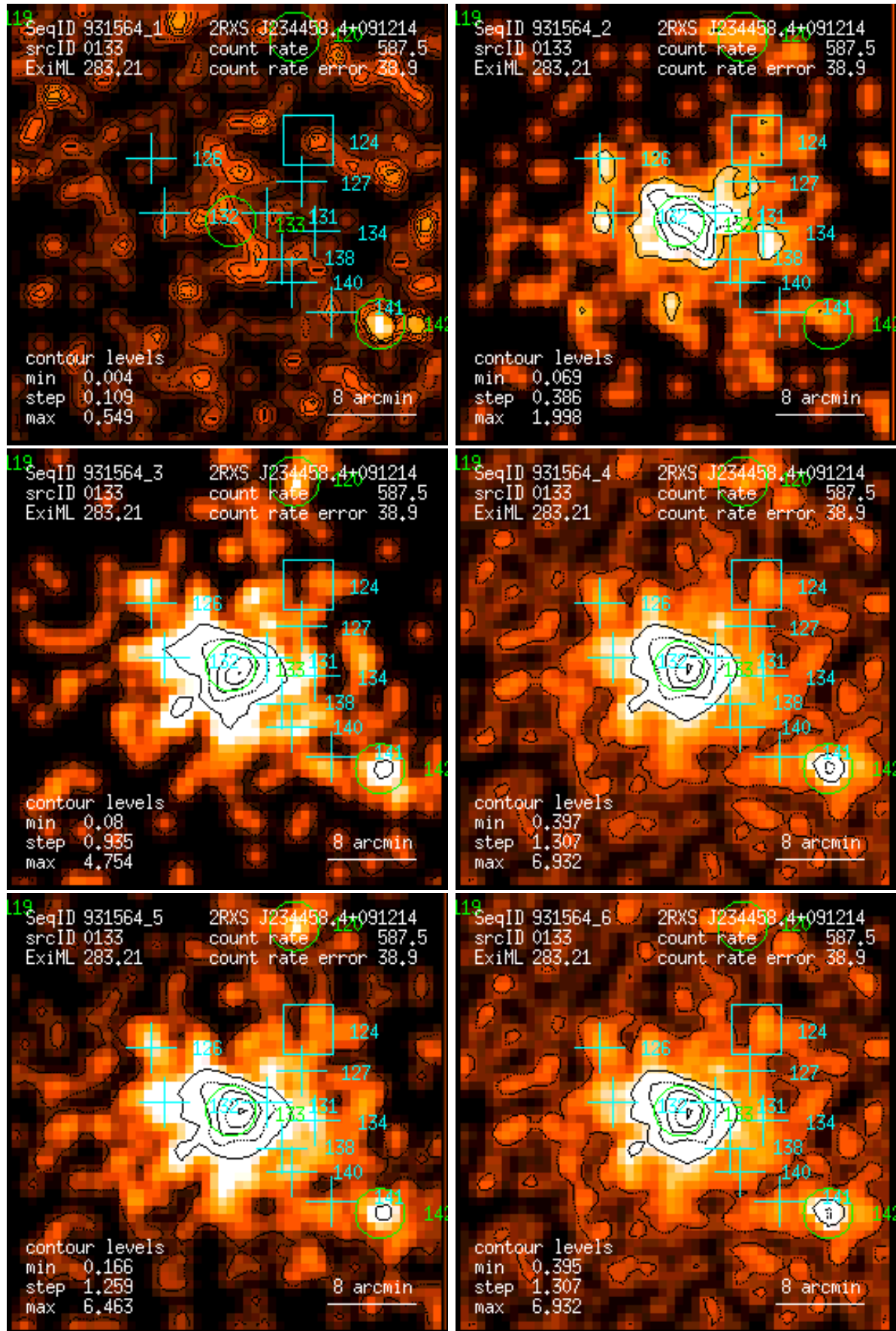
Figure 133: RASS 931564: detection 0133: band rate images, Gaussian filter: (1) PSPC channels 11 – 41, (2) 52 – 90, (3) 91 – 201, (4) 11 – 235, (5) 52 – 201, (6) 11 – 201. Broad band rates in counts/ks. Band rate contour levels in counts/ks/arcmin 2 .
