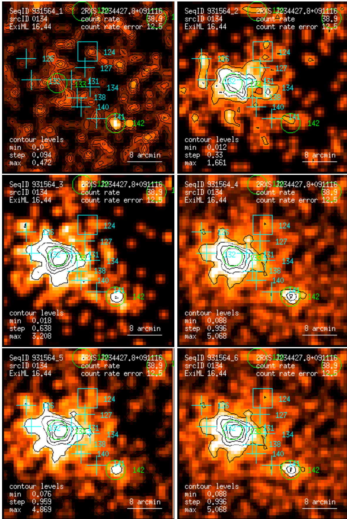
Figure 134: RASS 931564: detection 0134: band rate images, Gaussian filter: (1) PSPC channels 11 – 41, (2) 52 – 90, (3) 91 – 201, (4) 11 – 235, (5) 52 – 201, (6) 11 – 201. Broad band rates in counts/ks. Band rate contour levels in counts/ks/arcmin 2 .
