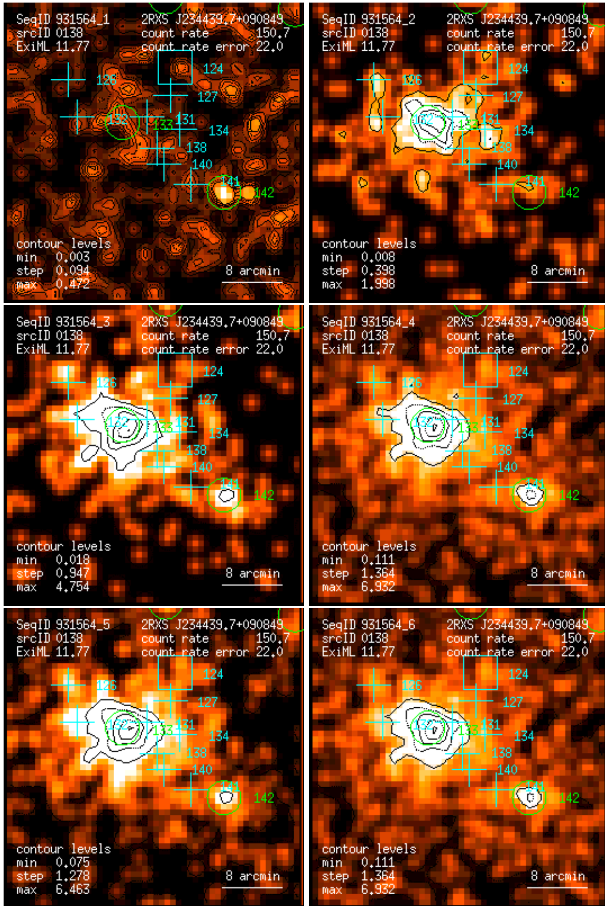
Figure 138: RASS 931564: detection 0138: band rate images, Gaussian filter: (1) PSPC channels 11 – 41, (2) 52 – 90, (3) 91 – 201, (4) 11 – 235, (5) 52 – 201, (6) 11 – 201. Broad band rates in counts/ks. Band rate contour levels in counts/ks/arcmin 2 .
