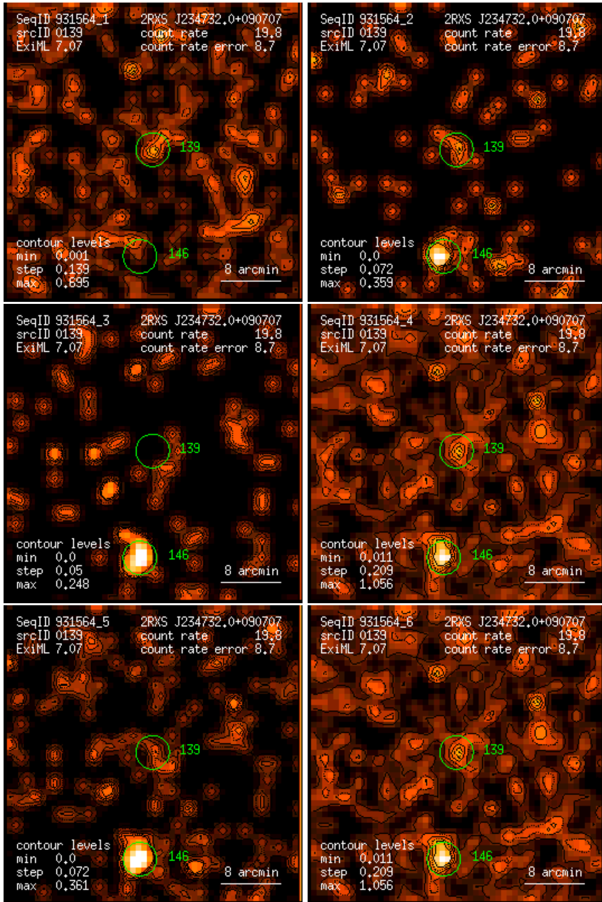
Figure 139: RASS 931564: detection 0139: band rate images, Gaussian filter: (1) PSPC channels 11 – 41, (2) 52 – 90, (3) 91 – 201, (4) 11 – 235, (5) 52 – 201, (6) 11 – 201. Broad band rates in counts/ks. Band rate contour levels in counts/ks/arcmin 2 .
