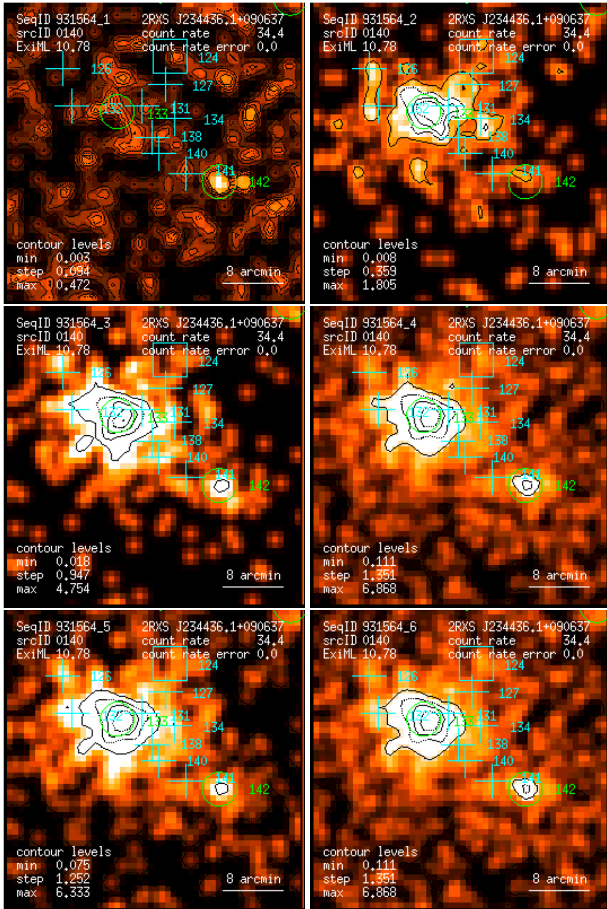
Figure 140: RASS 931564: detection 0140: band rate images, Gaussian filter: (1) PSPC channels 11 – 41, (2) 52 – 90, (3) 91 – 201, (4) 11 – 235, (5) 52 – 201, (6) 11 – 201. Broad band rates in counts/ks. Band rate contour levels in counts/ks/arcmin 2 .
