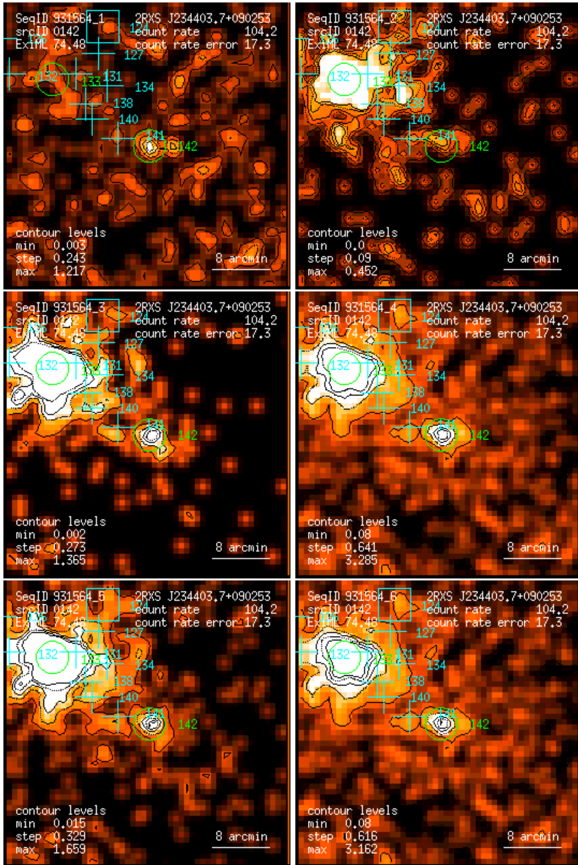
Figure 142: RASS 931564: detection 0142: band rate images, Gaussian filter: (1) PSPC channels 11 – 41, (2) 52 – 90, (3) 91 – 201, (4) 11 – 235, (5) 52 – 201, (6) 11 – 201. Broad band rates in counts/ks. Band rate contour levels in counts/ks/arcmin 2 .
