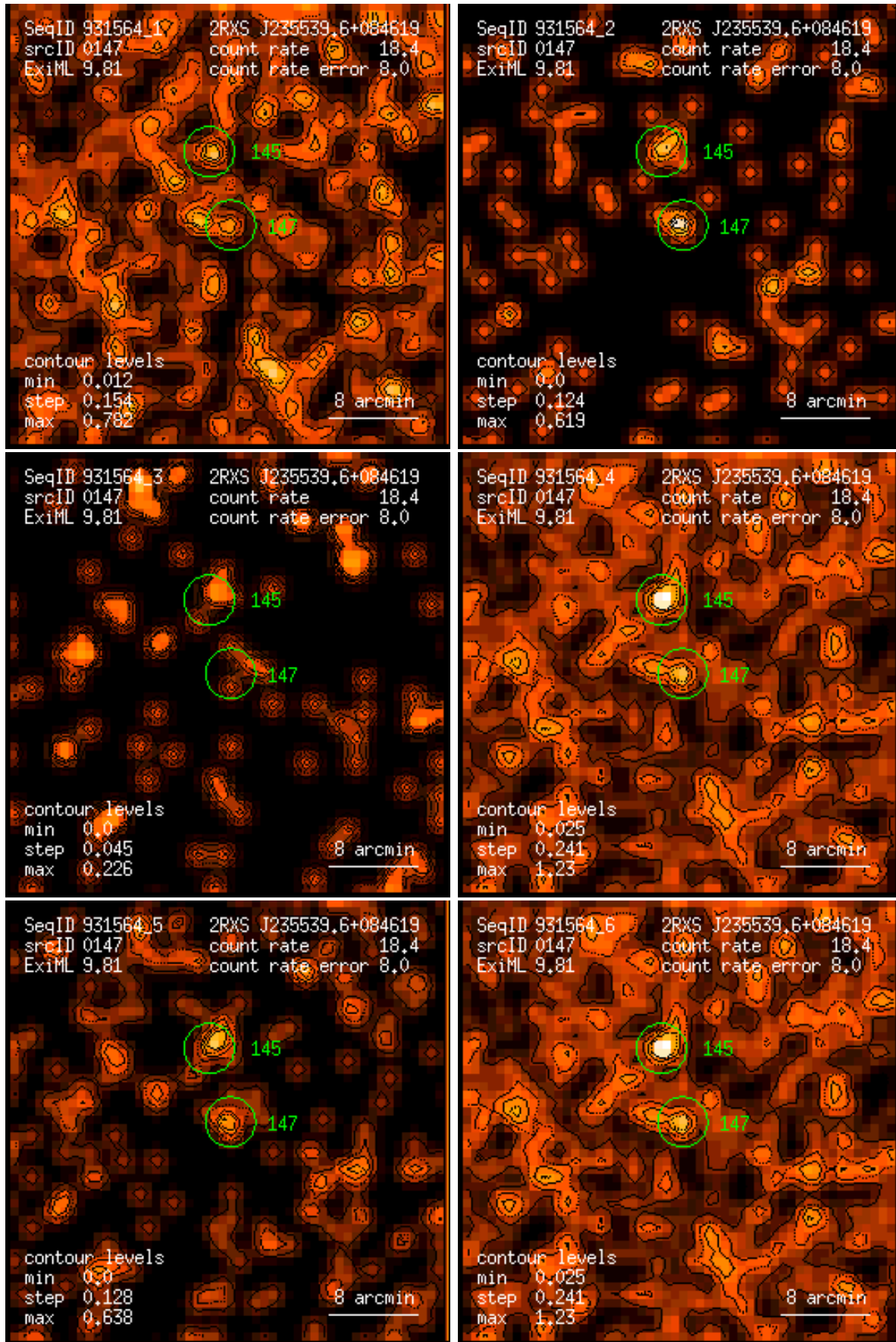
Figure 147: RASS 931564: detection 0147: band rate images, Gaussian filter: (1) PSPC channels 11 – 41, (2) 52 – 90, (3) 91 – 201, (4) 11 – 235, (5) 52 – 201, (6) 11 – 201. Broad band rates in counts/ks. Band rate contour levels in counts/ks/arcmin 2 .
