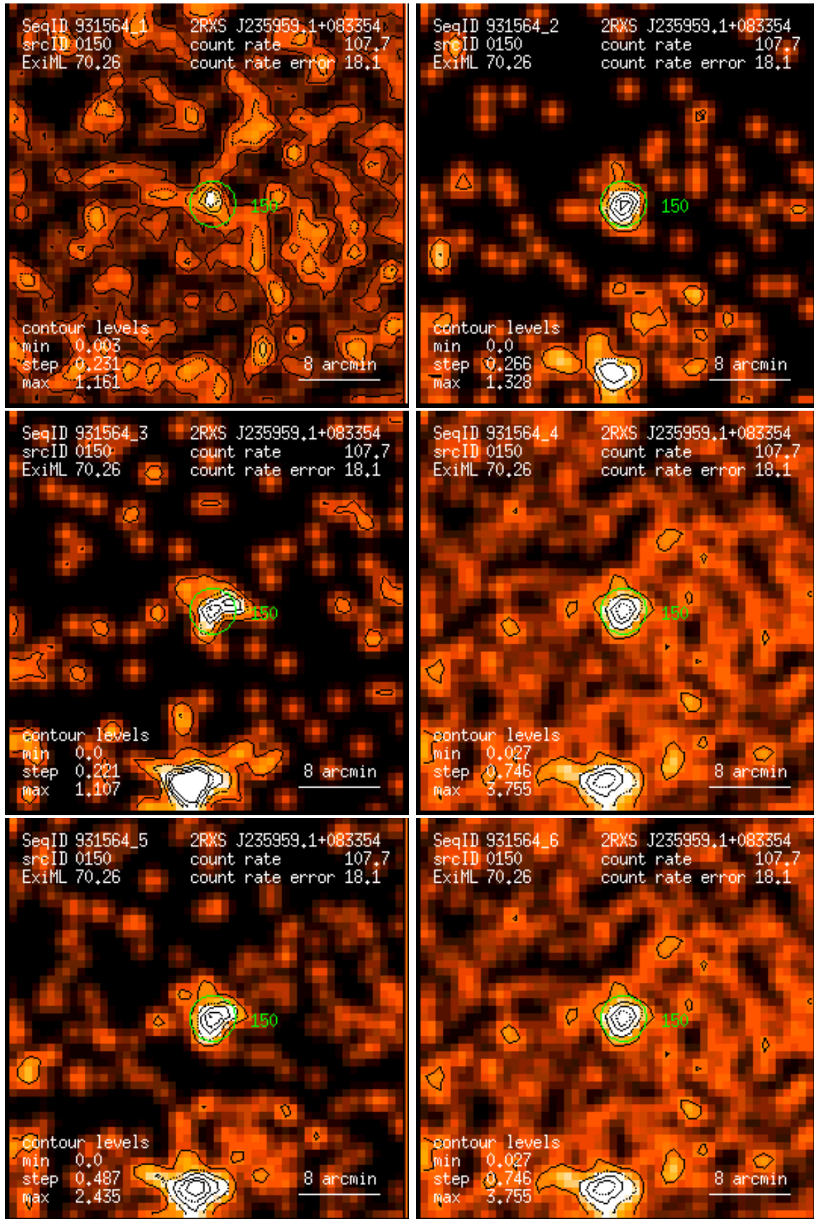
Figure 150: RASS 931564: detection 0150: band rate images, Gaussian filter: (1) PSPC channels 11 – 41, (2) 52 – 90, (3) 91 – 201, (4) 11 – 235, (5) 52 – 201, (6) 11 – 201. Broad band rates in counts/ks. Band rate contour levels in counts/ks/arcmin 2 .
