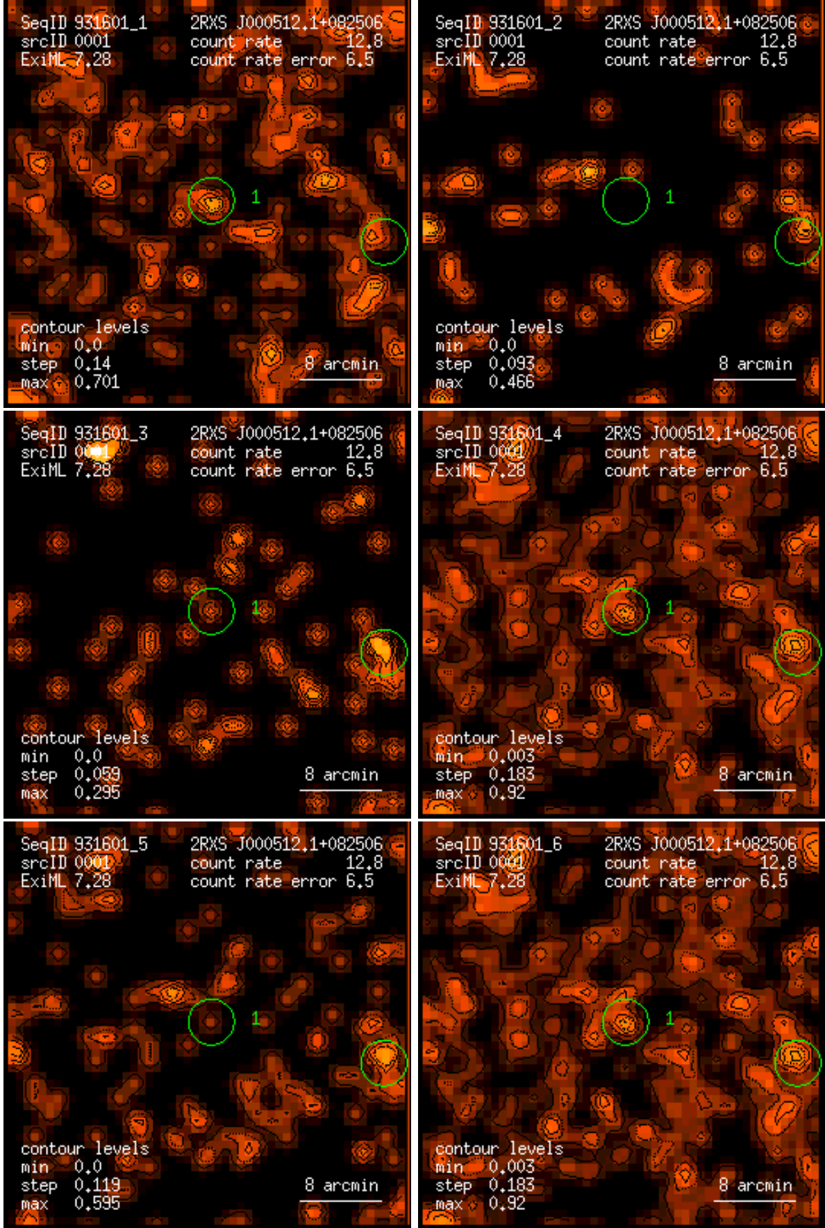
Figure 1: RASS 931601: detection 0001: band rate images, Gaussian filter: (1) PSPC channels 11 – 41, (2) 52 – 90, (3) 91 – 201, (4) 11 – 235, (5) 52 – 201, (6) 11 – 201. Broad band rates in counts/ks. Band rate contour levels in counts/ks/arcmin 2 .
