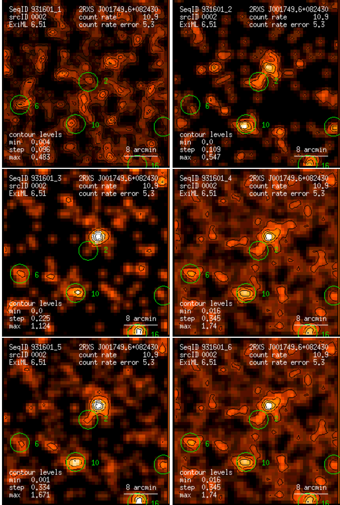
Figure 2: RASS 931601: detection 0002: band rate images, Gaussian filter: (1) PSPC channels 11 – 41, (2) 52 – 90, (3) 91 – 201, (4) 11 – 235, (5) 52 – 201, (6) 11 – 201. Broad band rates in counts/ks. Band rate contour levels in counts/ks/arcmin 2 .
