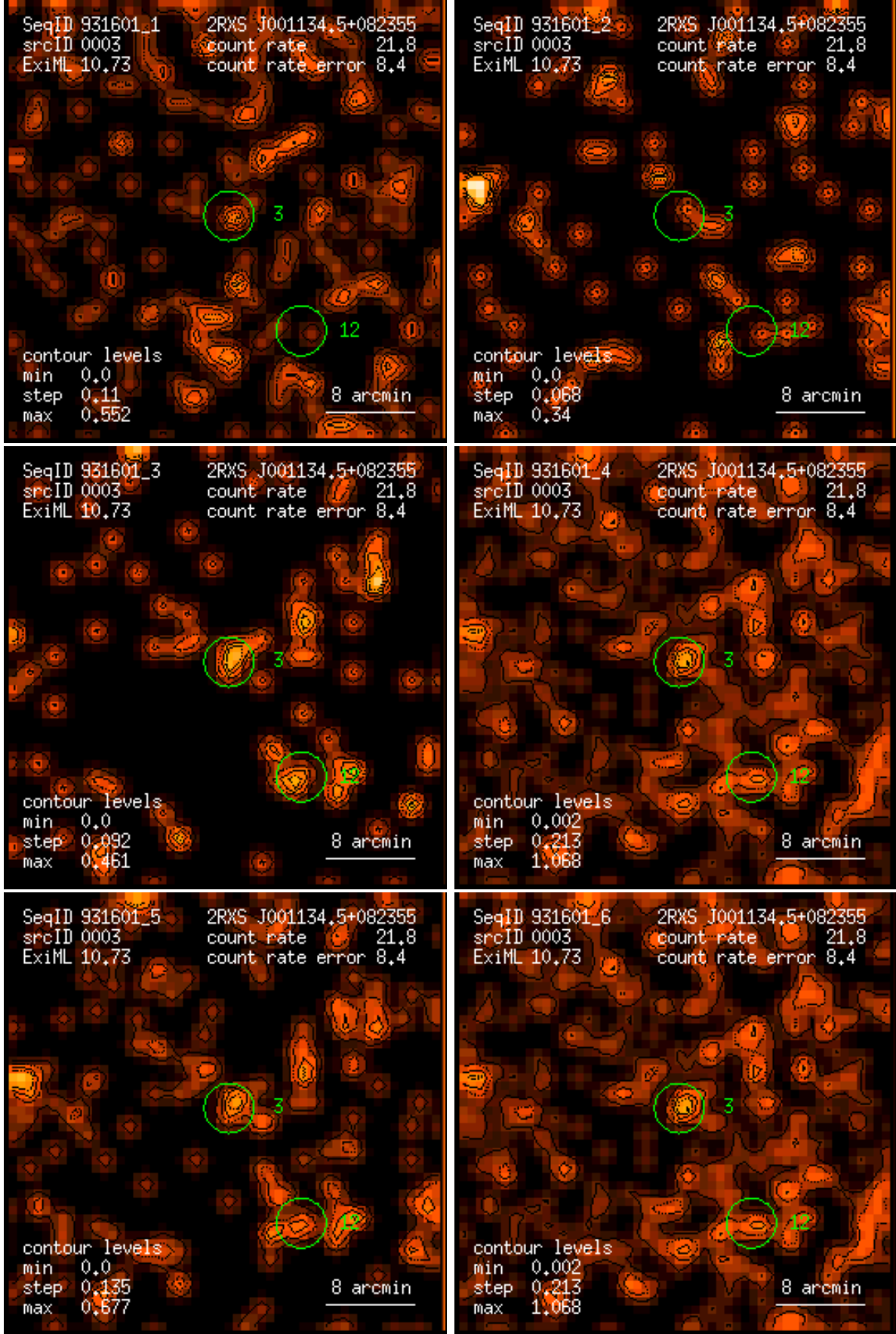
Figure 3: RASS 931601: detection 0003: band rate images, Gaussian filter: (1) PSPC channels 11 – 41, (2) 52 – 90, (3) 91 – 201, (4) 11 – 235, (5) 52 – 201, (6) 11 – 201. Broad band rates in counts/ks. Band rate contour levels in counts/ks/arcmin 2 .
