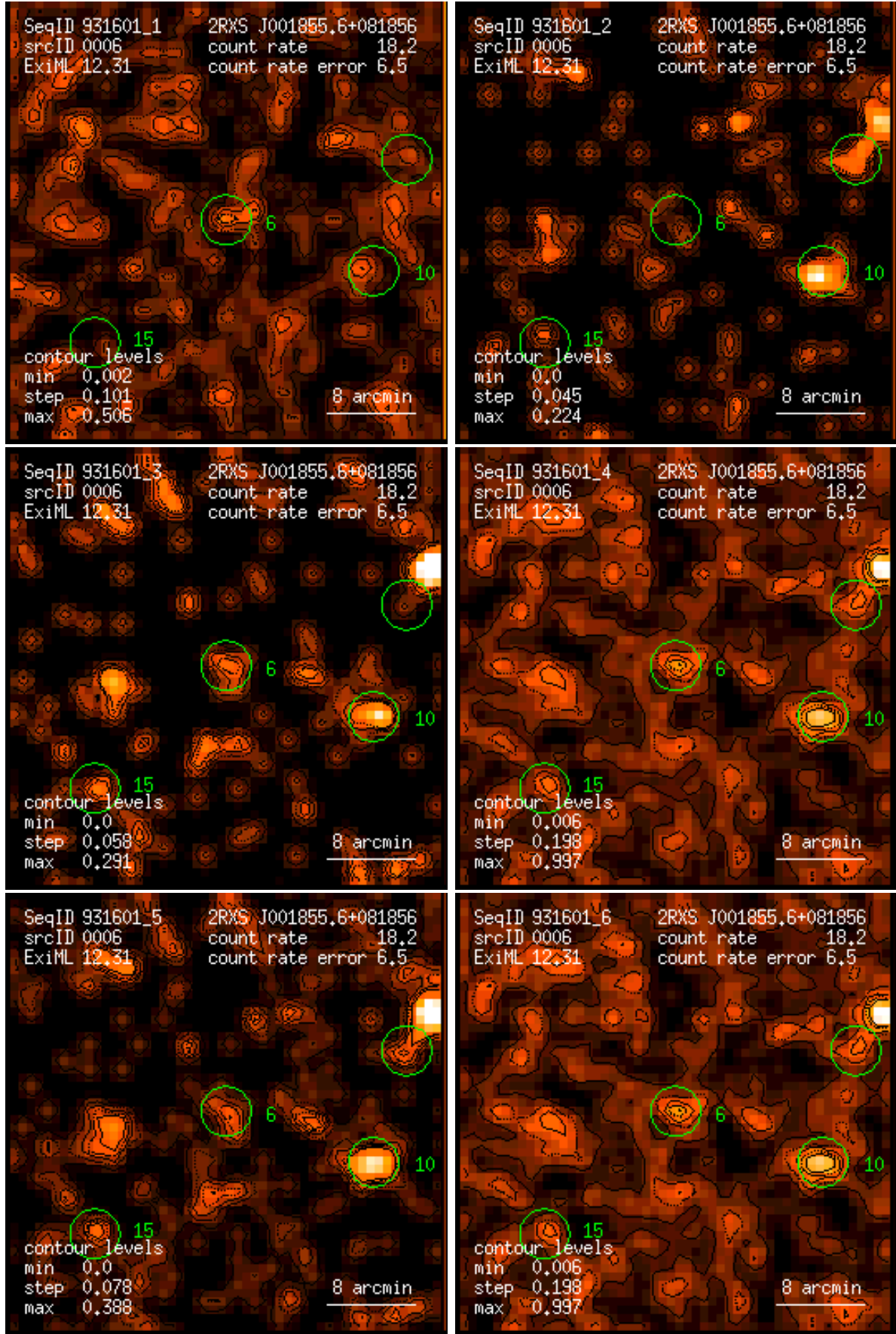
Figure 6: RASS 931601: detection 0006: band rate images, Gaussian filter: (1) PSPC channels 11 – 41, (2) 52 – 90, (3) 91 – 201, (4) 11 – 235, (5) 52 – 201, (6) 11 – 201. Broad band rates in counts/ks. Band rate contour levels in counts/ks/arcmin 2 .
