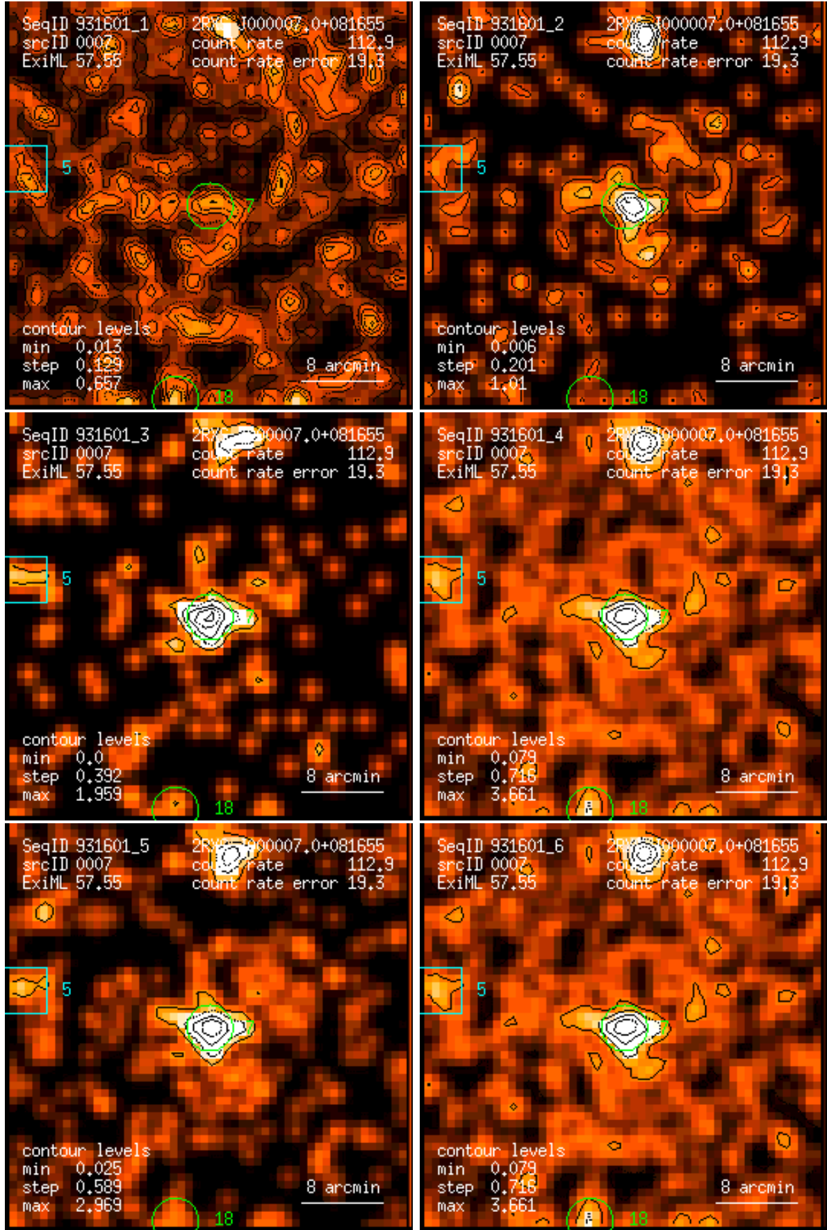
Figure 7: RASS 931601: detection 0007: band rate images, Gaussian filter: (1) PSPC channels 11 – 41, (2) 52 – 90, (3) 91 – 201, (4) 11 – 235, (5) 52 – 201, (6) 11 – 201. Broad band rates in counts/ks. Band rate contour levels in counts/ks/arcmin 2 .
