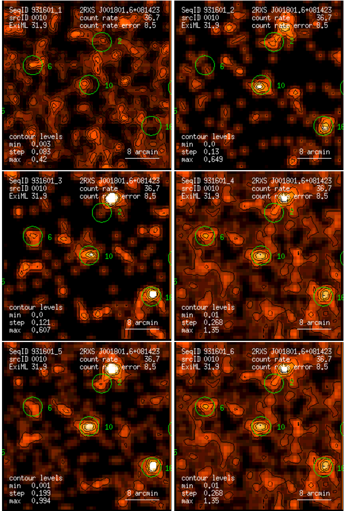
Figure 10: RASS 931601: detection 0010: band rate images, Gaussian filter: (1) PSPC channels 11 – 41, (2) 52 – 90, (3) 91 – 201, (4) 11 – 235, (5) 52 – 201, (6) 11 – 201. Broad band rates in counts/ks. Band rate contour levels in counts/ks/arcmin 2 .
