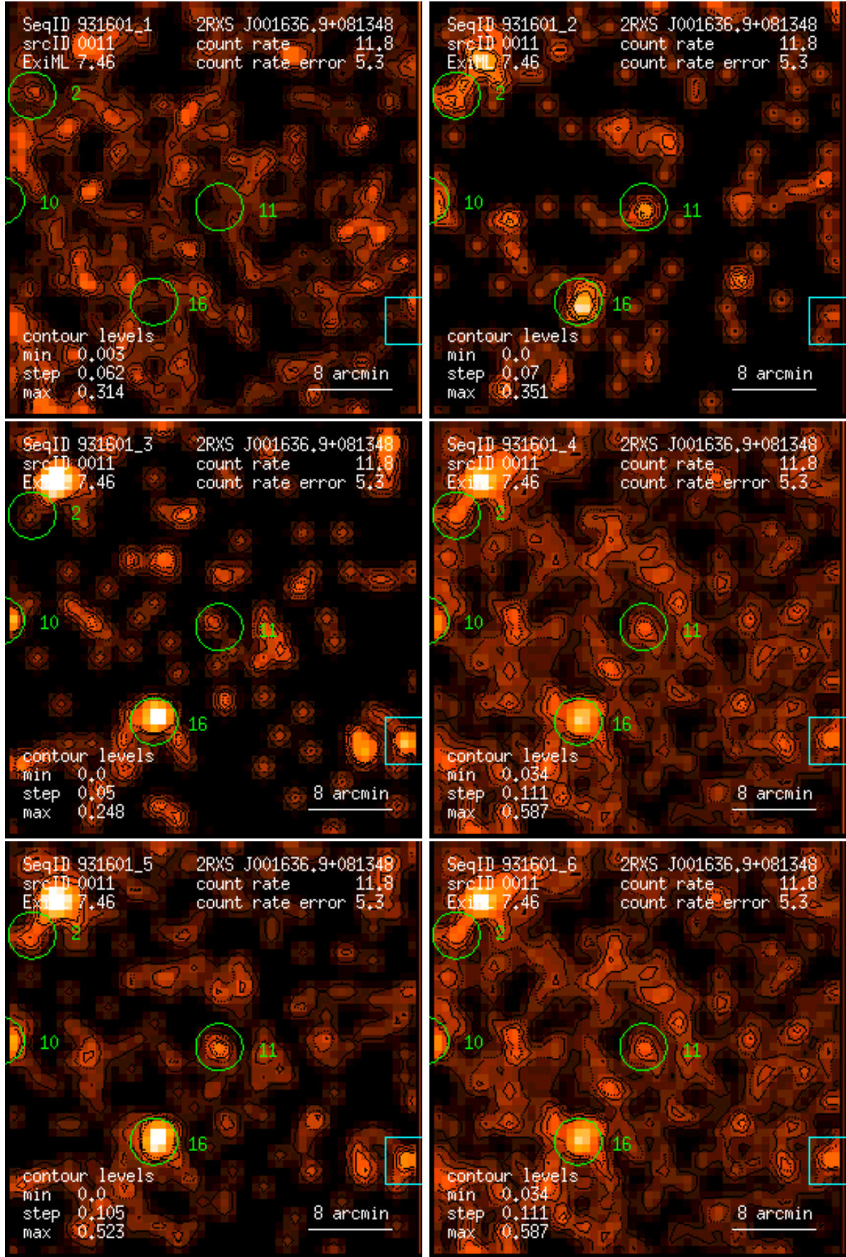
Figure 11: RASS 931601: detection 0011: band rate images, Gaussian filter: (1) PSPC channels 11 – 41, (2) 52 – 90, (3) 91 – 201, (4) 11 – 235, (5) 52 – 201, (6) 11 – 201. Broad band rates in counts/ks. Band rate contour levels in counts/ks/arcmin 2 .
