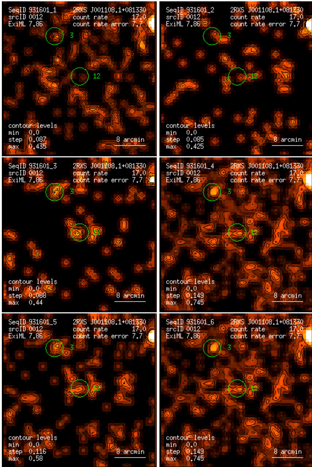
Figure 12: RASS 931601: detection 0012: band rate images, Gaussian filter: (1) PSPC channels 11 – 41, (2) 52 – 90, (3) 91 – 201, (4) 11 – 235, (5) 52 – 201, (6) 11 – 201. Broad band rates in counts/ks. Band rate contour levels in counts/ks/arcmin 2 .
