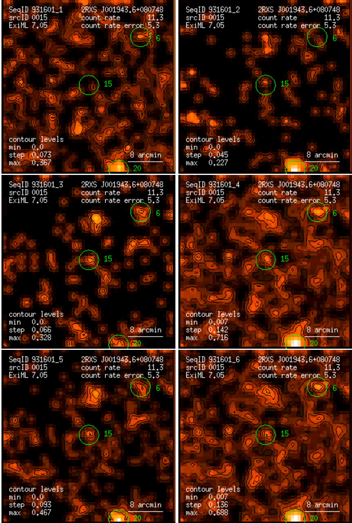
Figure 15: RASS 931601: detection 0015: band rate images, Gaussian filter: (1) PSPC channels 11 – 41, (2) 52 – 90, (3) 91 – 201, (4) 11 – 235, (5) 52 – 201, (6) 11 – 201. Broad band rates in counts/ks. Band rate contour levels in counts/ks/arcmin 2 .
