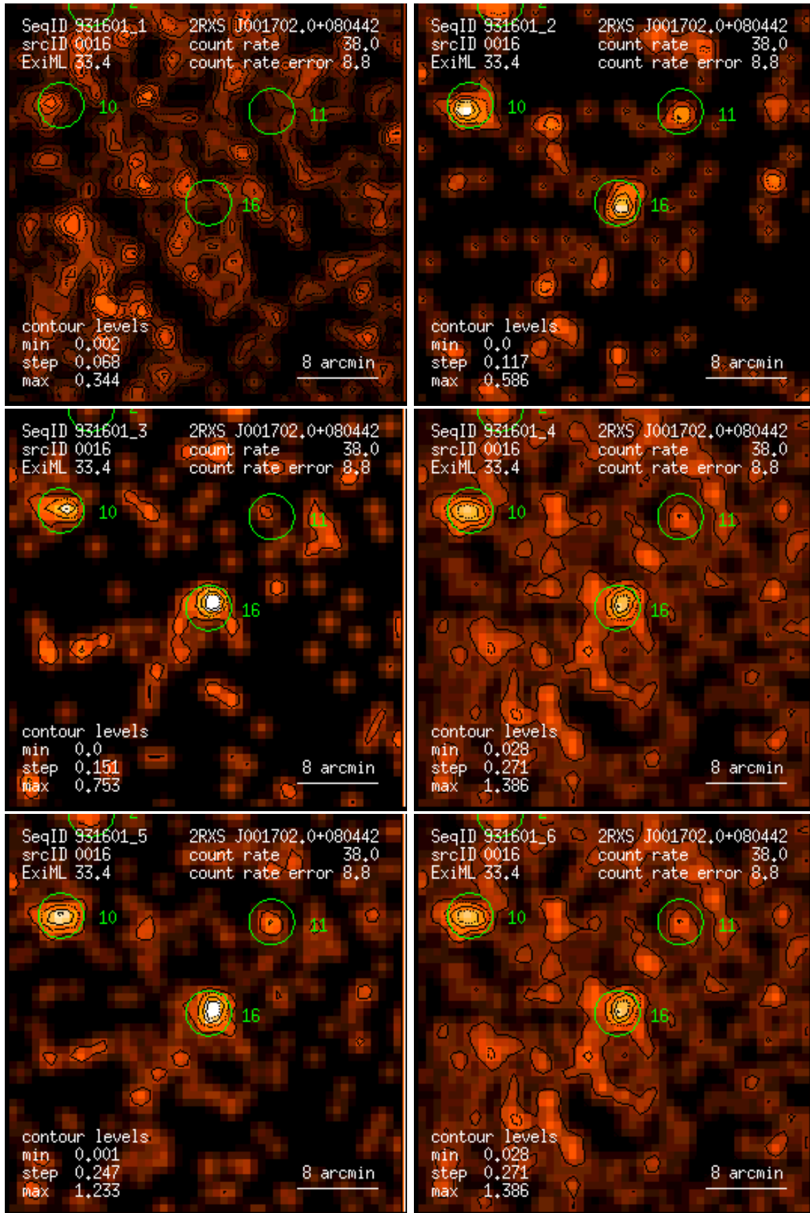
Figure 16: RASS 931601: detection 0016: band rate images, Gaussian filter: (1) PSPP channels 11 – 41, (2) 52 – 90, (3) 91 – 201, (4) 11 – 235, (5) 52 – 201, (6) 11 – 201. Broad band rates in counts/ks. Band rate contour levels in counts/ks/arcmin 2 .
