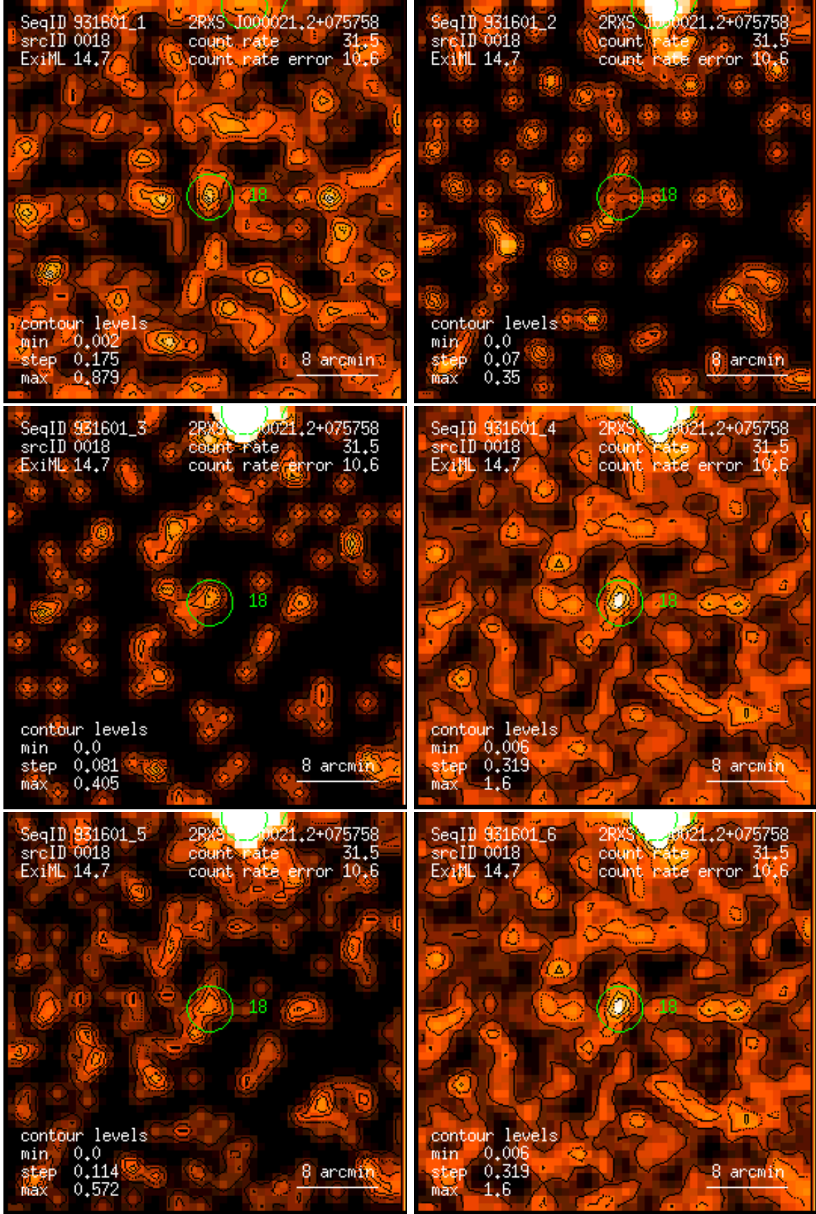
Figure 18: RASS 931601: detection 0018: band rate images, Gaussian filter: (1) PSPC channels 11 – 41, (2) 52 – 90, (3) 91 – 201, (4) 11 – 235, (5) 52 – 201, (6) 11 – 201. Broad band rates in counts/ks. Band rate contour levels in counts/ks/arcmin 2 .
