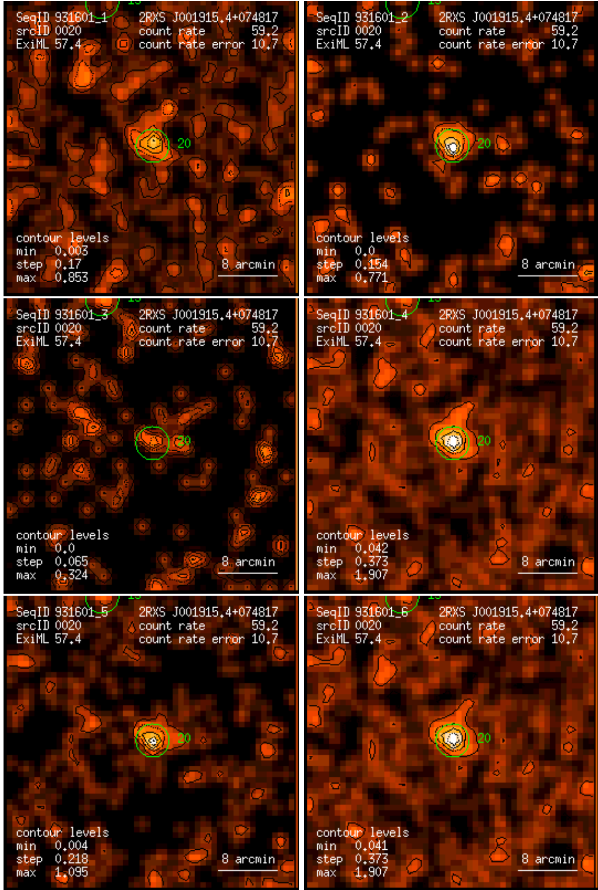
Figure 20: RASS 931601: detection 0020: band rate images, Gaussian filter: (1) PSPC channels 11 – 41, (2) 52 – 90, (3) 91 – 201, (4) 11 – 235, (5) 52 – 201, (6) 11 – 201. Broad band rates in counts/ks. Band rate contour levels in counts/ks/arcmin 2 .
