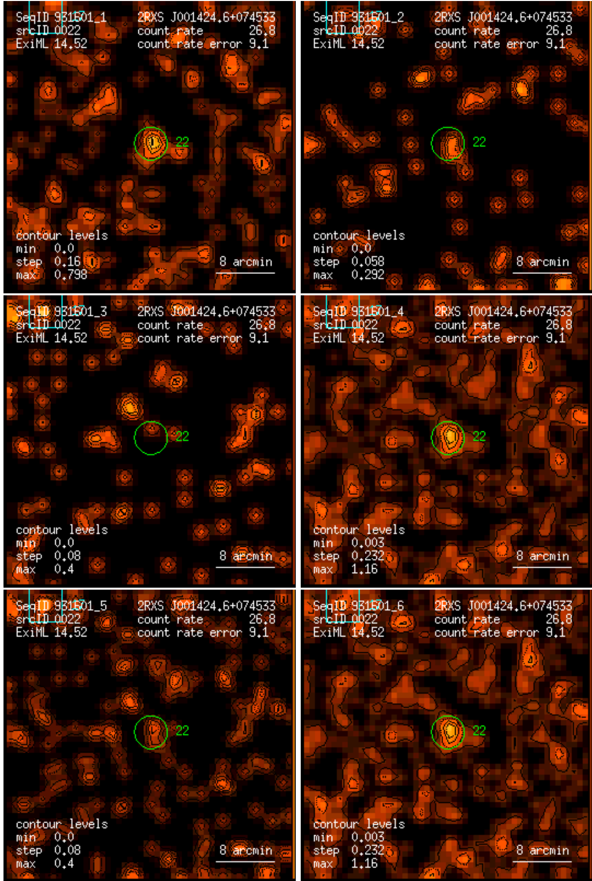
Figure 22: RASS 931601: detection 0022: band rate images, Gaussian filter: (1) PSPC channels 11 – 41, (2) 52 – 90, (3) 91 – 201, (4) 11 – 235, (5) 52 – 201, (6) 11 – 201. Broad band rates in counts/ks. Band rate contour levels in counts/ks/arcmin 2 .
