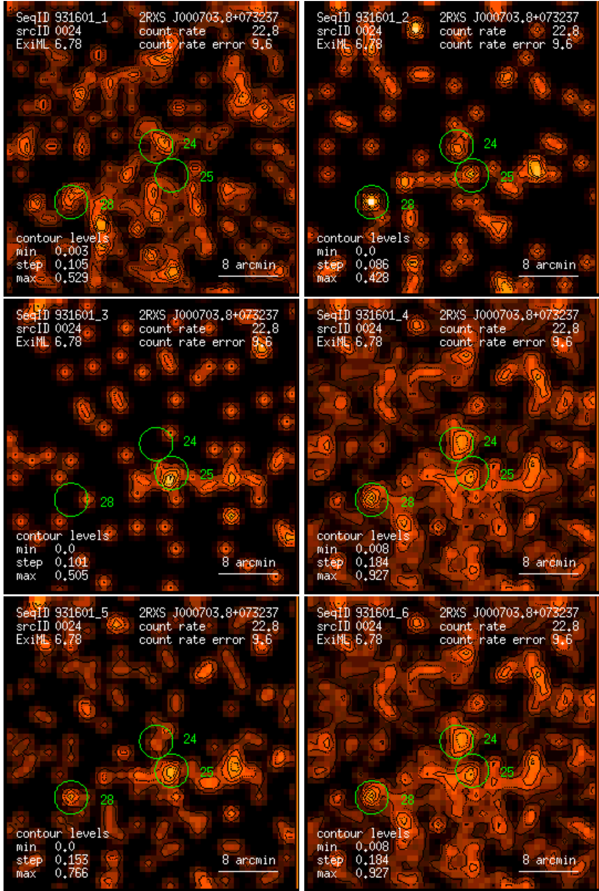
Figure 24: RASS 931601: detection 0024: band rate images, Gaussian filter: (1) PSPC channels 11 – 41, (2) 52 – 90, (3) 91 – 201, (4) 11 – 235, (5) 52 – 201, (6) 11 – 201. Broad band rates in counts/ks. Band rate contour levels in counts/ks/arcmin 2 .
