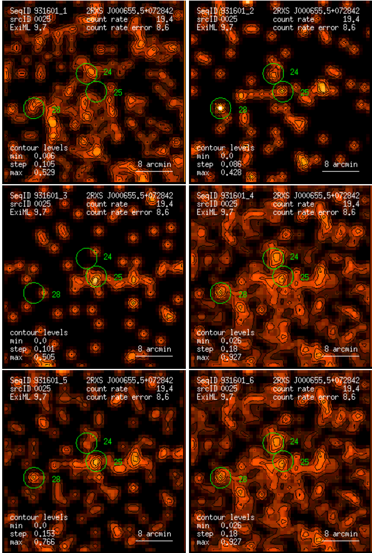
Figure 25: RASS 931601: detection 0025: band rate images, Gaussian filter: (1) PSPC channels 11 – 41, (2) 52 – 90, (3) 91 – 201, (4) 11 – 235, (5) 52 – 201, (6) 11 – 201. Broad band rates in counts/ks. Band rate contour levels in counts/ks/arcmin 2 .
