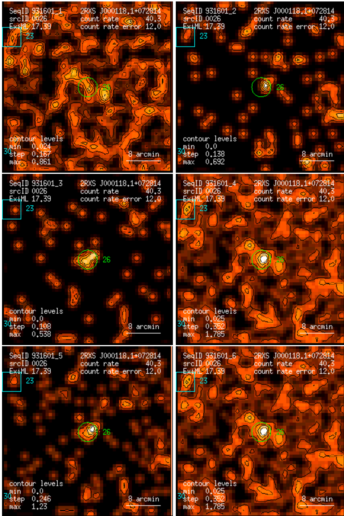
Figure 26: RASS 931601: detection 0026: band rate images, Gaussian filter: (1) PSPC channels 11 – 41, (2) 52 – 90, (3) 91 – 201, (4) 11 – 235, (5) 52 – 201, (6) 11 – 201. Broad band rates in counts/ks. Band rate contour levels in counts/ks/arcmin 2 .
