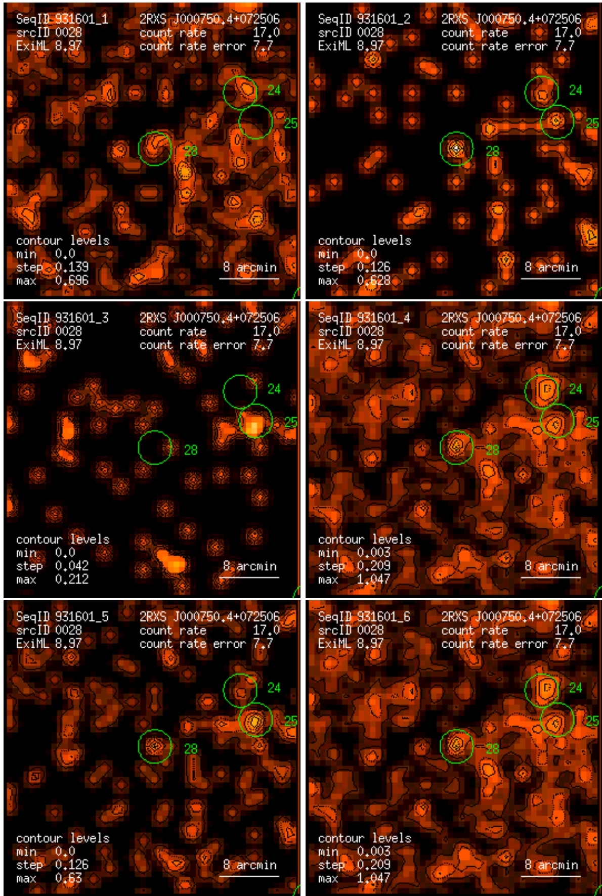
Figure 28: RASS 931601: detection 0028: band rate images, Gaussian filter: (1) PSPC channels 11 – 41, (2) 52 – 90, (3) 91 – 201, (4) 11 – 235, (5) 52 – 201, (6) 11 – 201. Broad band rates in counts/ks. Band rate contour levels in counts/ks/arcmin 2 .
