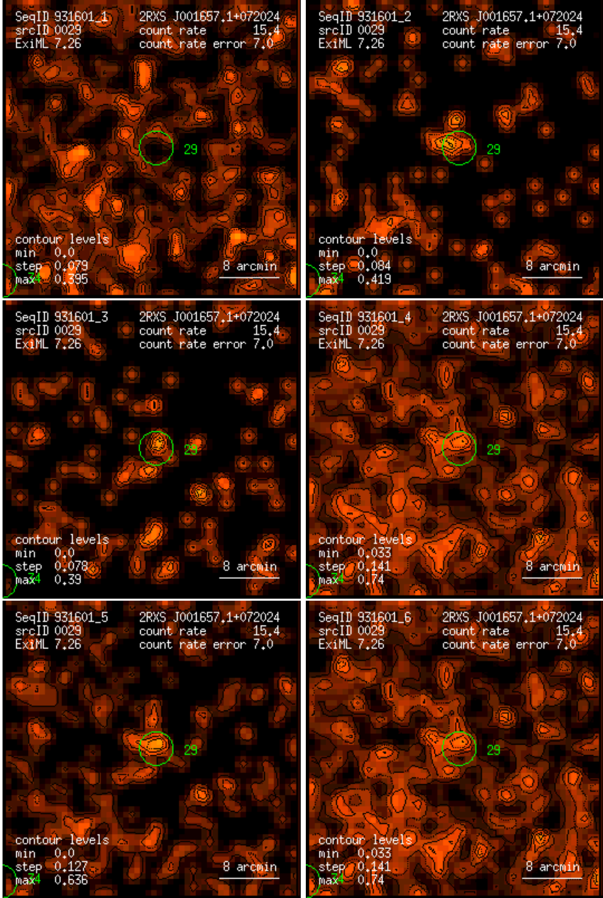
Figure 29: RASS 931601: detection 0029: band rate images, Gaussian filter: (1) PSPC channels 11 – 41, (2) 52 – 90, (3) 91 – 201, (4) 11 – 235, (5) 52 – 201, (6) 11 – 201. Broad band rates in counts/ks. Band rate contour levels in counts/ks/arcmin 2 .
