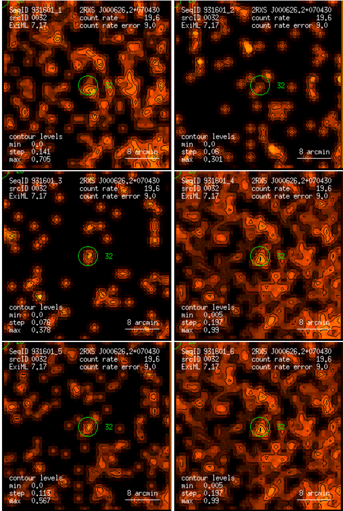
Figure 32: RASS 931601: detection 0032: band rate images, Gaussian filter: (1) PSPC channels 11 – 41, (2) 52 – 90, (3) 91 – 201, (4) 11 – 235, (5) 52 – 201, (6) 11 – 201. Broad band rates in counts/ks. Band rate contour levels in counts/ks/arcmin 2 .
