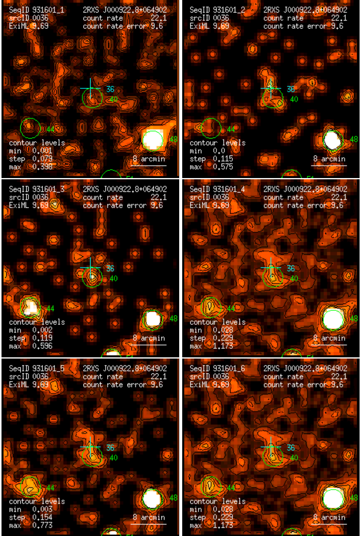
Figure 36: RASS 931601: detection 0036: band rate images, Gaussian filter: (1) PSPC channels 11 – 41, (2) 52 – 90, (3) 91 – 201, (4) 11 – 235, (5) 52 – 201, (6) 11 – 201. Broad band rates in counts/ks. Band rate contour levels in counts/ks/arcmin 2 .
