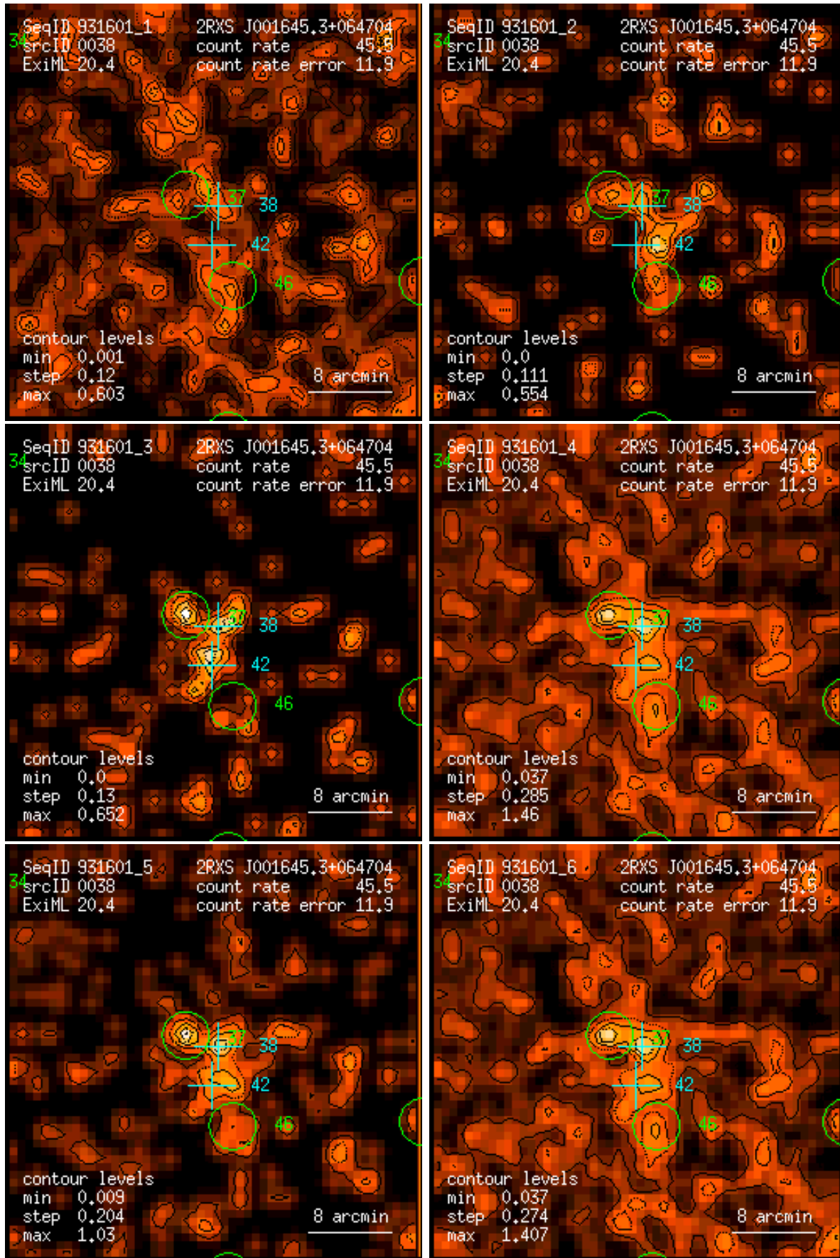
Figure 38: RASS 931601: detection 0038: band rate images, Gaussian filter: (1) PSPC channels 11 – 41, (2) 52 – 90, (3) 91 – 201, (4) 11 – 235, (5) 52 – 201, (6) 11 – 201. Broad band rates in counts/ks. Band rate contour levels in counts/ks/arcmin 2 .
