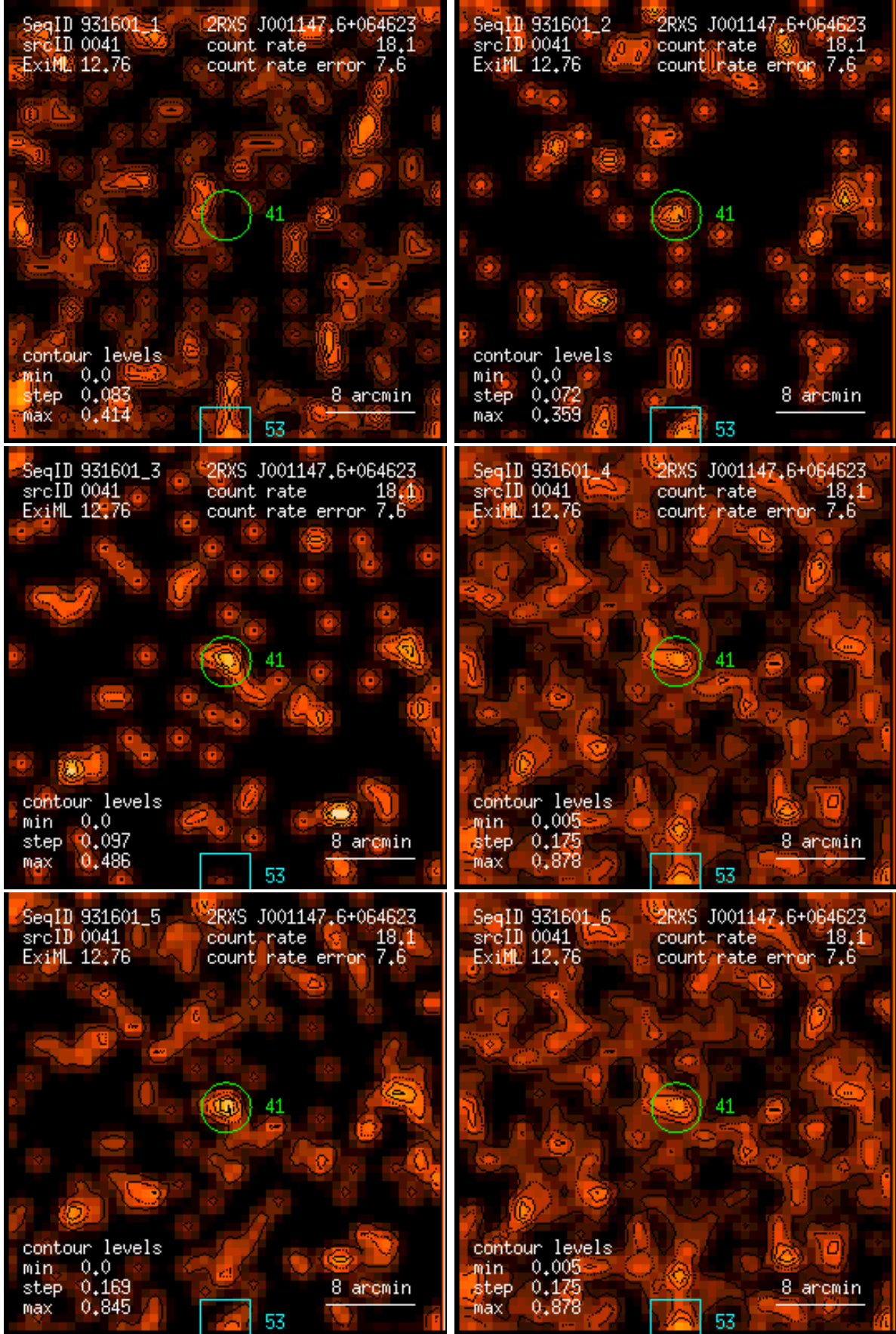
Figure 41: RASS 931601: detection 0041: band rate images, Gaussian filter: (1) PSPC channels 11 – 41, (2) 52 – 90, (3) 91 – 201, (4) 11 – 235, (5) 52 – 201, (6) 11 – 201. Broad band rates in counts/ks. Band rate contour levels in counts/ks/arcmin 2 .
