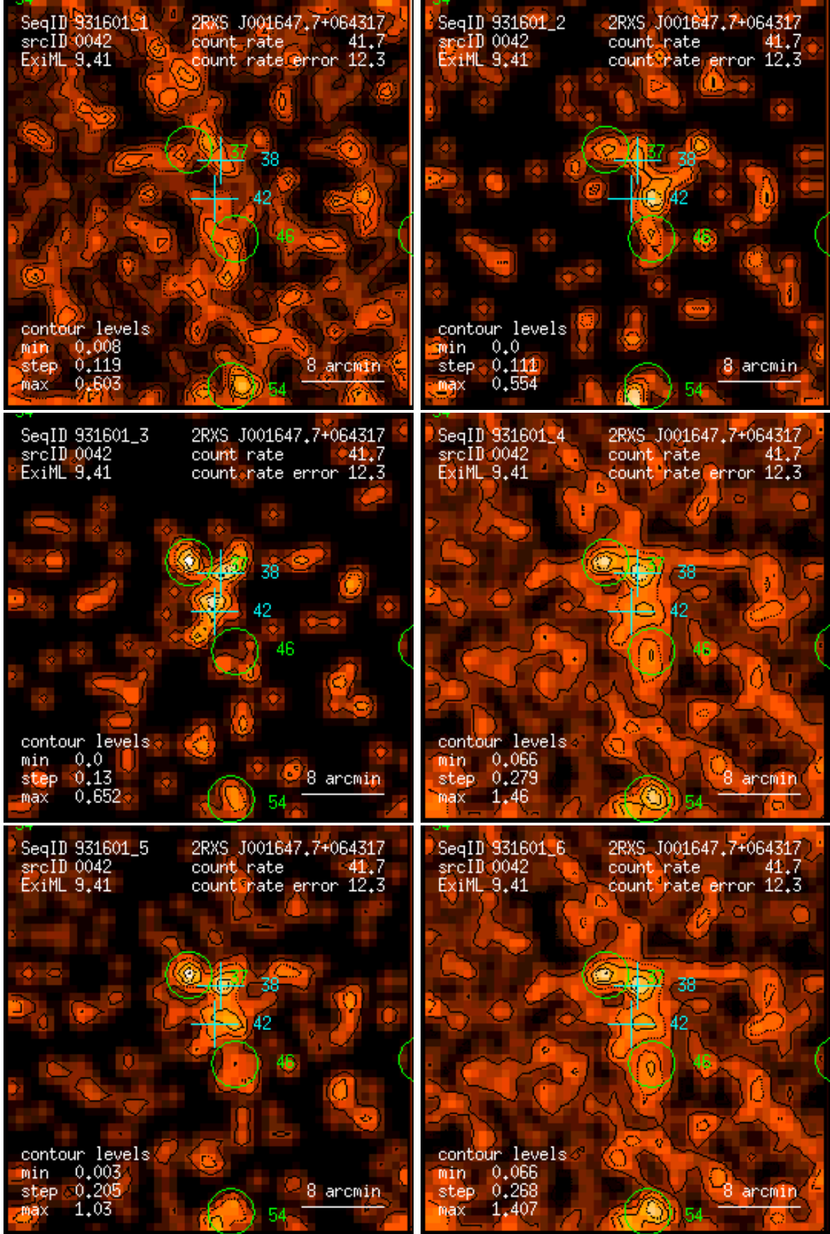
Figure 42: RASS 931601: detection 0042: band rate images, Gaussian filter: (1) PSPC channels 11 – 41, (2) 52 – 90, (3) 91 – 201, (4) 11 – 235, (5) 52 – 201, (6) 11 – 201. Broad band rates in counts/ks. Band rate contour levels in counts/ks/arcmin 2 .
