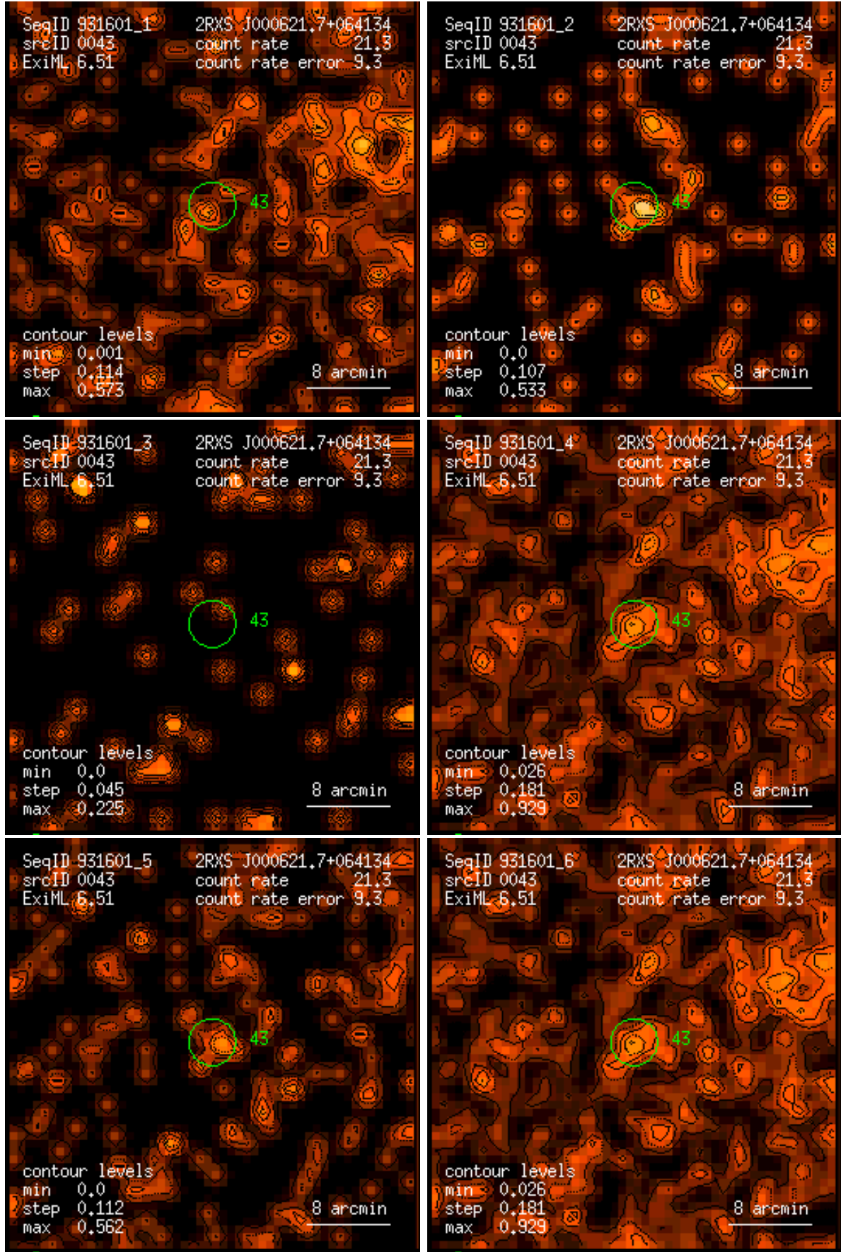
Figure 43: RASS 931601: detection 0043: band rate images, Gaussian filter: (1) PSPC channels 11 – 41, (2) 52 – 90, (3) 91 – 201, (4) 11 – 235, (5) 52 – 201, (6) 11 – 201. Broad band rates in counts/ks. Band rate contour levels in counts/ks/arcmin 2 .
