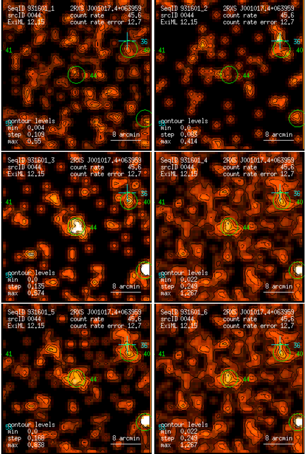
Figure 44: RASS 931601: detection 0044: band rate images, Gaussian filter: (1) PSPC channels 11 – 41, (2) 52 – 90, (3) 91 – 201, (4) 11 – 235, (5) 52 – 201, (6) 11 – 201. Broad band rates in counts/ks. Band rate contour levels in counts/ks/arcmin 2 .
