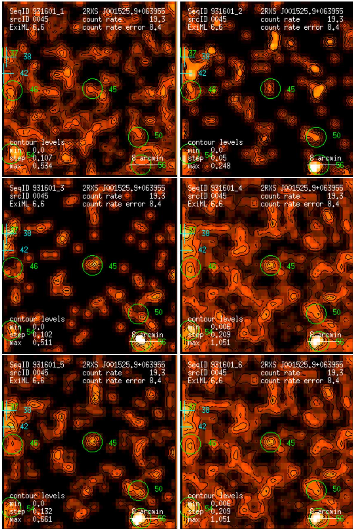
Figure 45: RASS 931601: detection 0045: band rate images, Gaussian filter: (1) PSPC channels 11 – 41, (2) 52 – 90, (3) 91 – 201, (4) 11 – 235, (5) 52 – 201, (6) 11 – 201. Broad band rates in counts/ks. Band rate contour levels in counts/ks/arcmin 2 .
