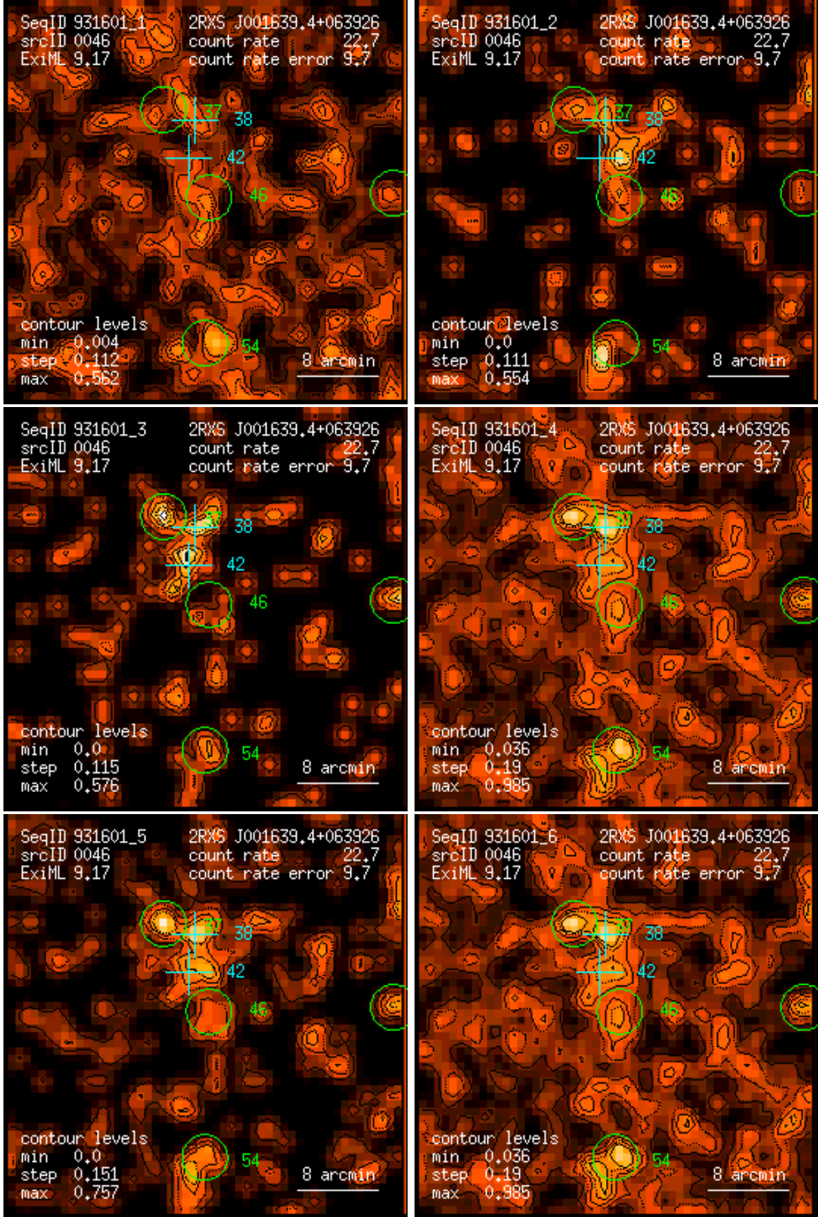
Figure 46: RASS 931601: detection 0046: band rate images, Gaussian filter: (1) PSPC channels 11 – 41, (2) 52 – 90, (3) 91 – 201, (4) 11 – 235, (5) 52 – 201, (6) 11 – 201. Broad band rates in counts/ks. Band rate contour levels in counts/ks/arcmin 2 .
