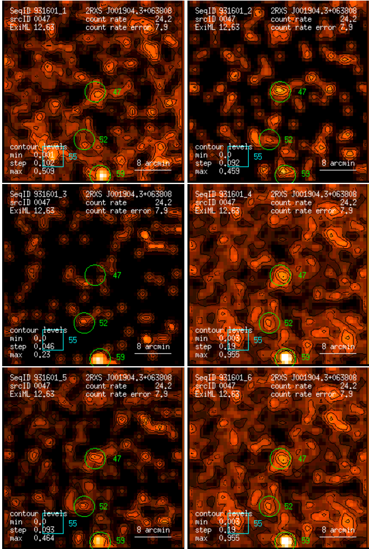
Figure 47: RASS 931601: detection 0047: band rate images, Gaussian filter: (1) PSPC channels 11 – 41, (2) 52 – 90, (3) 91 – 201, (4) 11 – 235, (5) 52 – 201, (6) 11 – 201. Broad band rates in counts/ks. Band rate contour levels in counts/ks/arcmin 2 .
