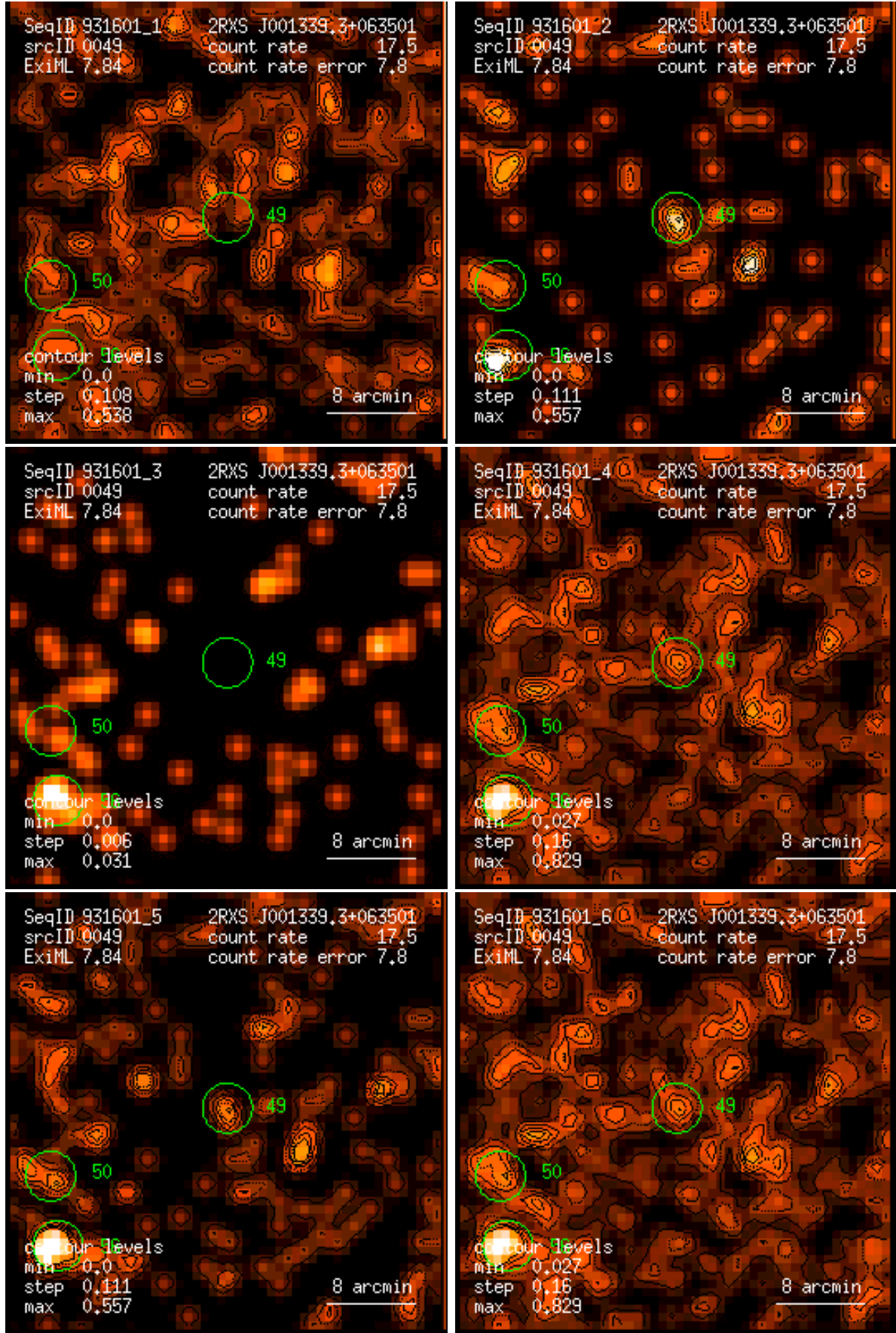
Figure 49: RASS 931601: detection 0049: band rate images, Gaussian filter: (1) PSPC channels 11 – 41, (2) 52 – 90, (3) 91 – 201, (4) 11 – 235, (5) 52 – 201, (6) 11 – 201. Broad band rates in counts/ks. Band rate contour levels in counts/ks/arcmin 2 .
