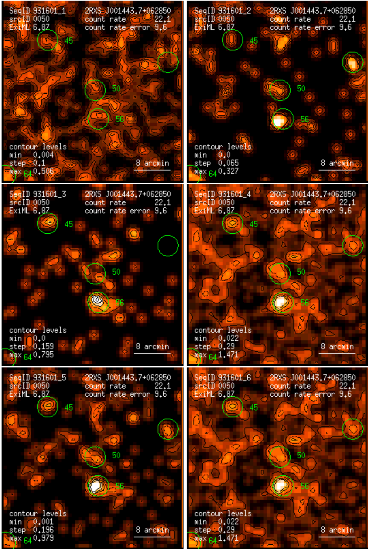
Figure 50: RASS 931601: detection 0050: band rate images, Gaussian filter: (1) PSPC channels 11 – 41, (2) 52 – 90, (3) 91 – 201, (4) 11 – 235, (5) 52 – 201, (6) 11 – 201. Broad band rates in counts/ks. Band rate contour levels in counts/ks/arcmin 2 .
