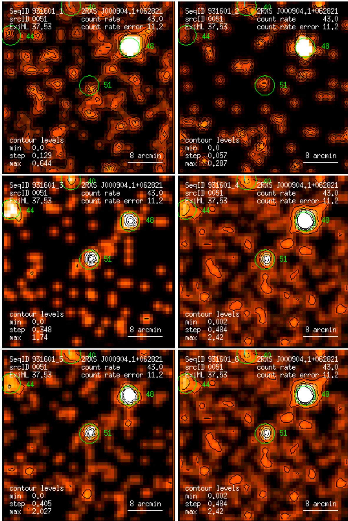
Figure 51: RASS 931601: detection 0051: band rate images, Gaussian filter: (1) PSPC channels 11 – 41, (2) 52 – 90, (3) 91 – 201, (4) 11 – 235, (5) 52 – 201, (6) 11 – 201. Broad band rates in counts/ks. Band rate contour levels in counts/ks/arcmin 2 .
