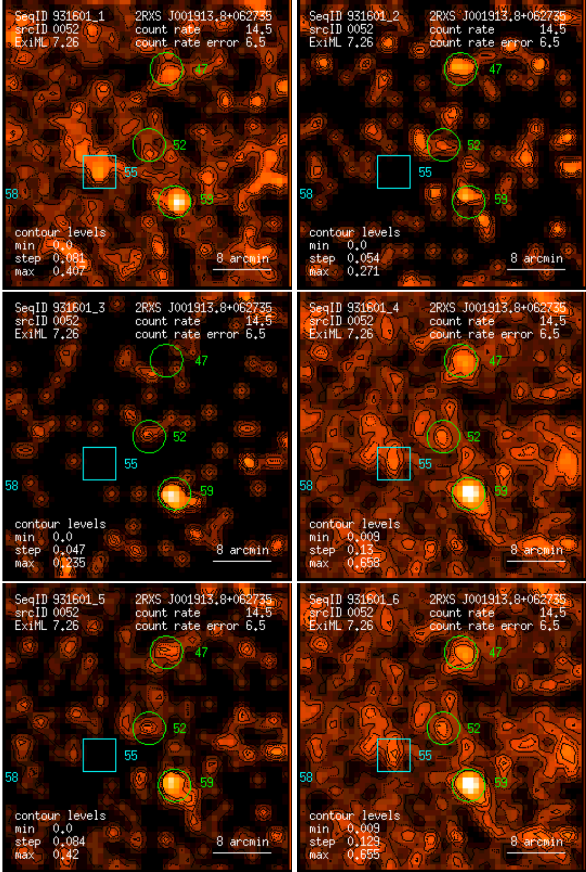
Figure 52: RASS 931601: detection 0052: band rate images, Gaussian filter: (1) PSPC channels 11 – 41, (2) 52 – 90, (3) 91 – 201, (4) 11 – 235, (5) 52 – 201, (6) 11 – 201. Broad band rates in counts/ks. Band rate contour levels in counts/ks/arcmin 2 .
