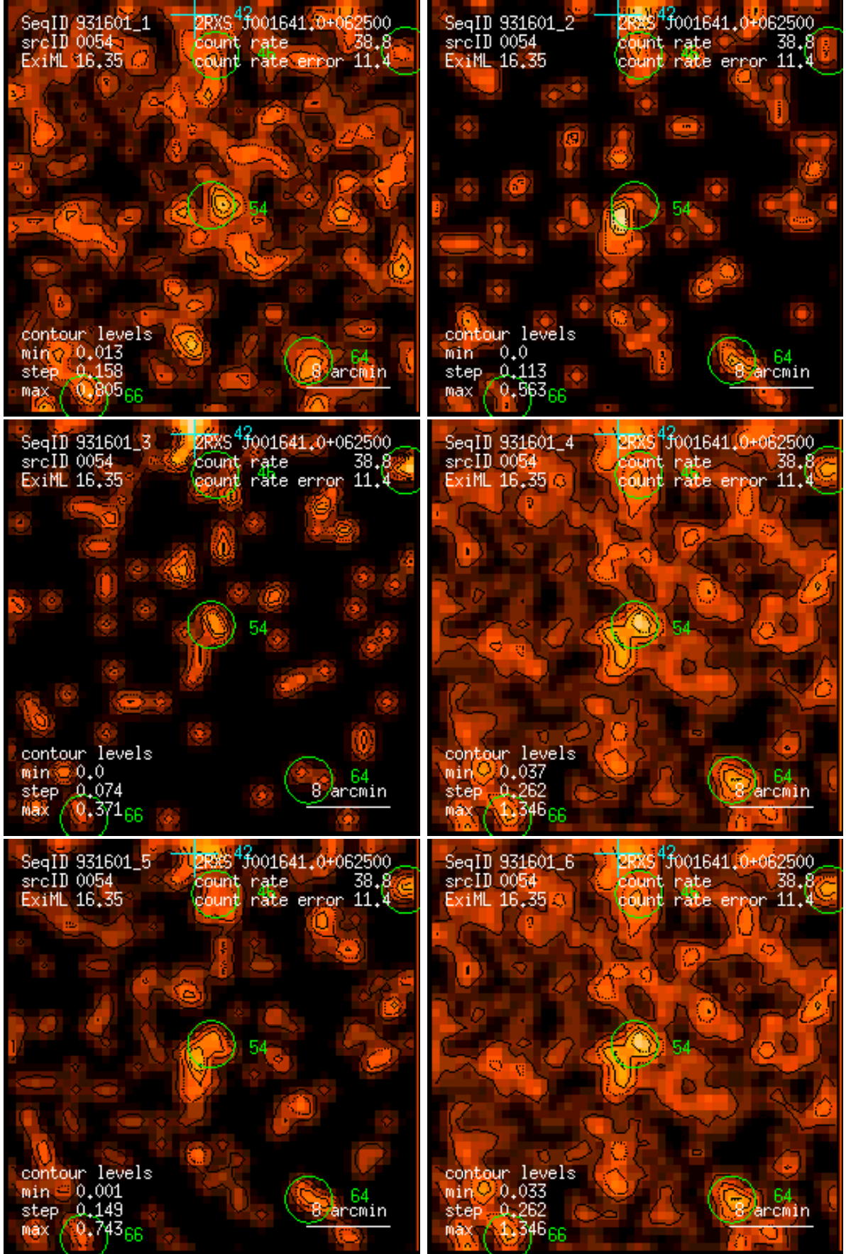
Figure 54: RASS 931601: detection 0054: band rate images, Gaussian filter: (1) PSPC channels 11 – 41, (2) 52 – 90, (3) 91 – 201, (4) 11 – 235, (5) 52 – 201, (6) 11 – 201. Broad band rates in counts/ks. Band rate contour levels in counts/ks/arcmin 2 .
